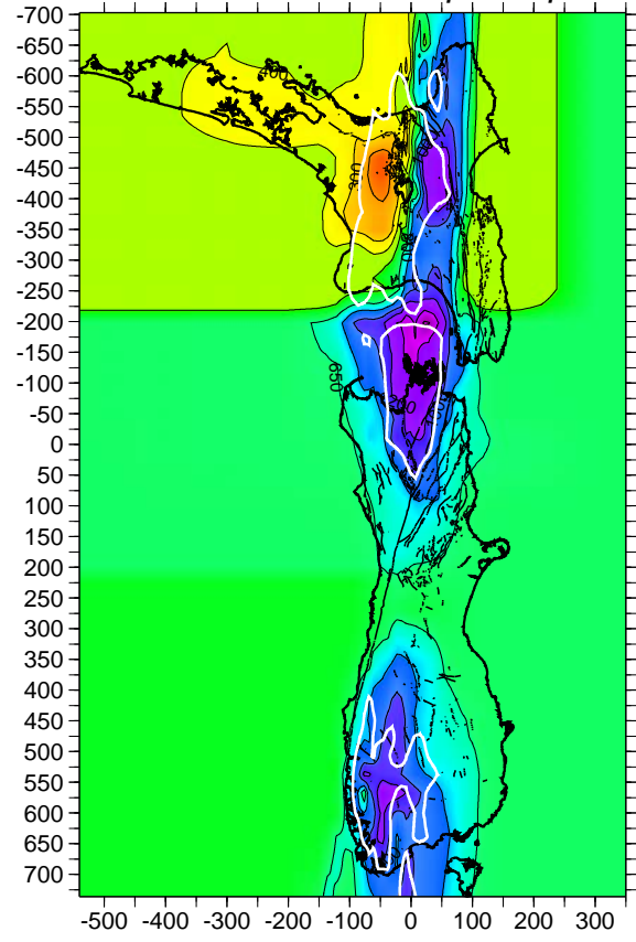
Z= 130 Qpnzw2p2
