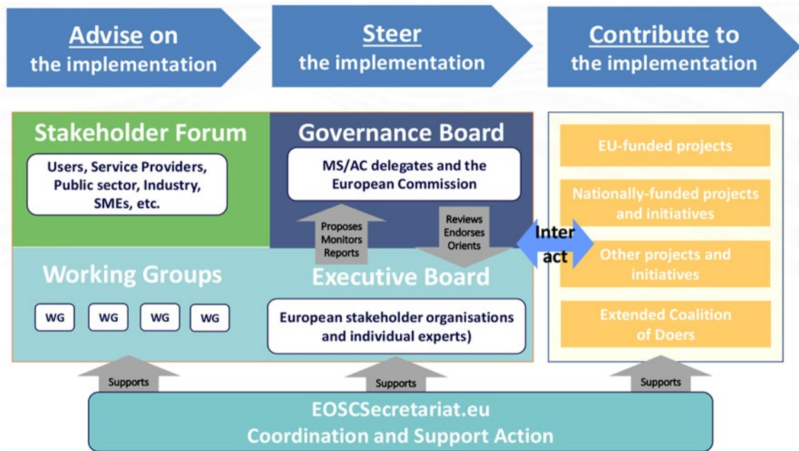
Figure 2: EOSC Governance 16
