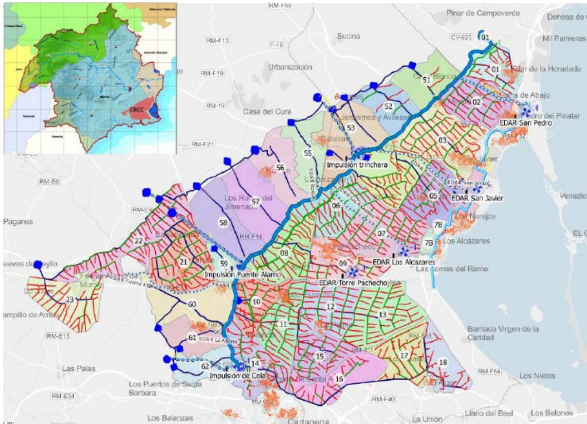
Figure 15. Irrigation piping network at Campo de Cartagena Source: Soto (2020)
