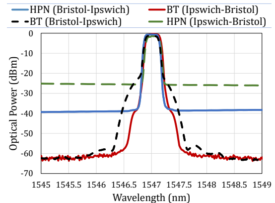
Fig. 7. Optical spectrum Bristol-Ipswich link
