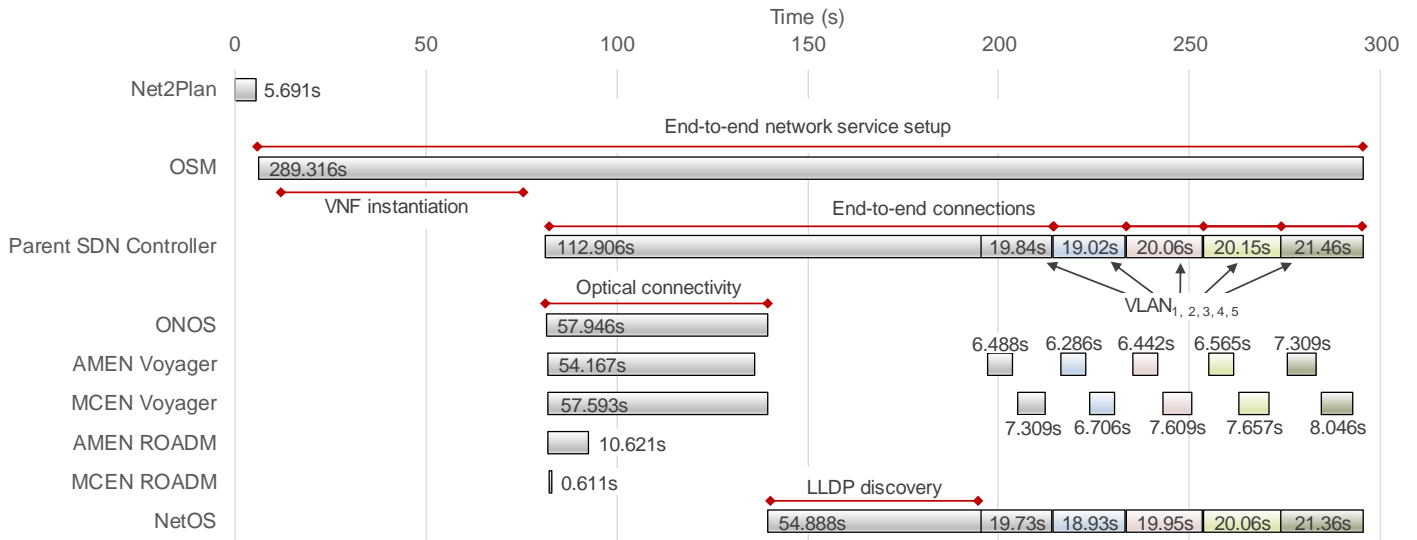
Fig. 6. Detailed setup times per Metro-Haul components. The times reflect one particular experiment run.
