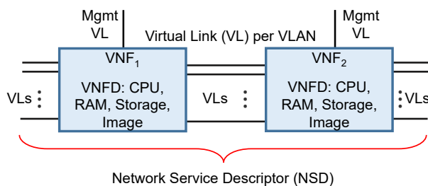
Fig. 4. ETSI-based Network Service Descriptor
