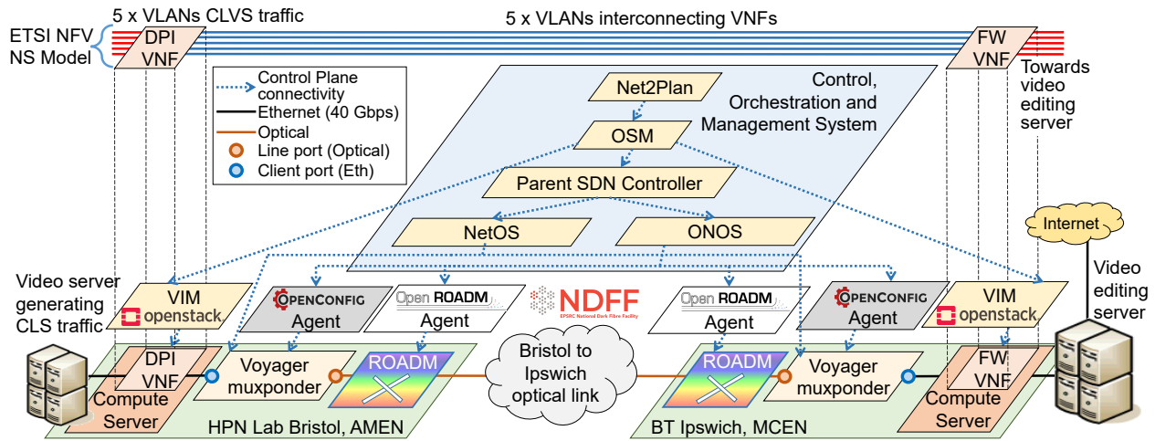
Fig. 2. Testbed for CLVS DPI application
