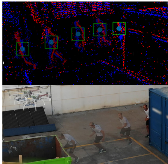
Fig. 1: Intrusion monitoring example of the proposed scheme in UAS-based experiments.
