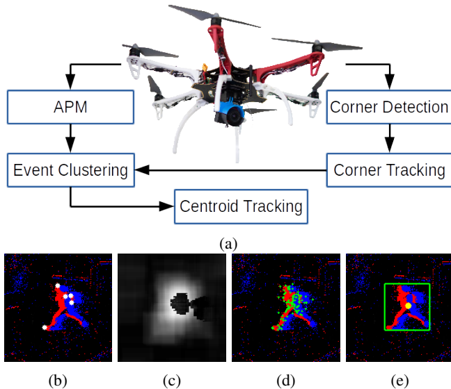
Fig. 2: (a) Scheme of the proposed asynchronous scheme. Results from each developed module: b) corner tracking, c) APM, d) event clustering and, e) intruder monitoring.
