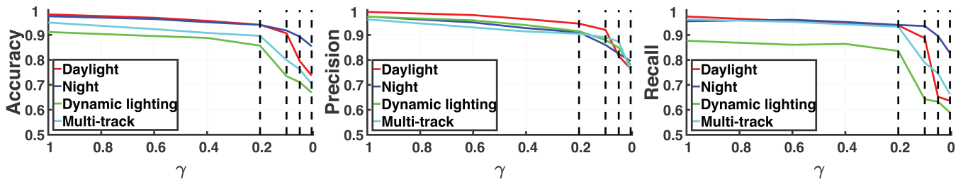
Fig. 4: Performance results for all experiments. Accuracy , Precision and Recall as a function of \gamma .
