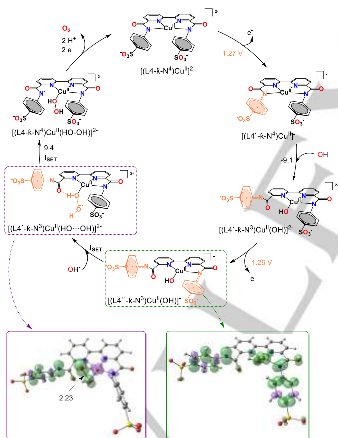
Figure 3. Catalytic cycle for [(L4)Cu]^{2-} ( [(L4-\kappa-N^4)Cu^{II}]^{2-} ) via the SET-WNA mechanism. Free energy changes are indicated in black in kcal·mol -1 and the calculated redox potentials are shown in orange in V vs. NHE. Spin densities are shown for selected intermediates. The radical character of the ligands is indicated in the formula.
