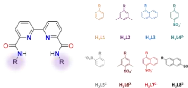
Figure 1. Drawings of H_2LN^{n-} ( N = 1-3 , n = 0 ; N = 4-8 ; n = 2 ) bpy-amidate ligands used in this work.
