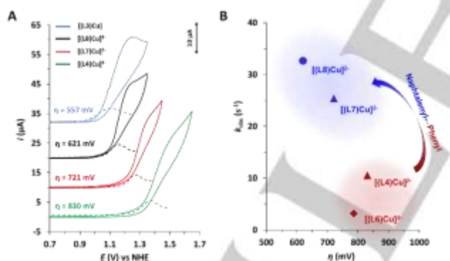
Figure 5. A, CVs of a 1 mM solution of [(L3)Cu] (blue line), [(L4)Cu]^{2-} (green line), [(L7)Cu]^{2-} (red line) and [(L8)Cu]^{2-} (black line) in 0.1 M phosphate buffer at pH 11.6. Note: In case of complex [(L3)Cu] the experiments were performed in a mixture of 0.1 M phosphate buffer/TFE (6:4) for solubility reasons. B, plot of k_{obs} ( s^{-1} ) for the water oxidation catalysis vs. \eta (mV) for selected cases.
