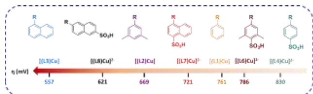
Figure 4. Influence of the substituents in [(LN)Cu]^{n-} ( n = 0 or 2 ) complexes on the \eta (mV) of the water oxidation reaction.
