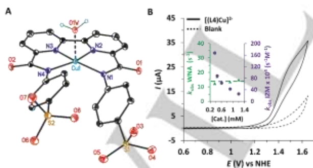
Figure 2. A, ORTEP drawing of [(L4)Cu]^{2-} at 50% probability level. The solvent molecules, sodium and hydrogen atoms have been omitted for clarity. Color code: C, black; N, blue; O, red; S, yellow; Cu, light blue. B, Cyclic Voltammogram of 1 mM solution of [(L4)Cu]^{2-} in 0.1 M phosphate buffer at pH 11.6 at scan rate of 100 mV/s. Inset: Plot of k_{obs} vs. [(L4)Cu]^{2-} calculated by FOWA analysis assuming a WNA mechanism (green trace) or an I2M mechanism (purple trace).
