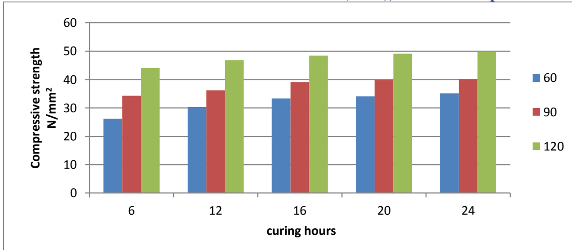
Fig 2 . 3 Days Compressive Strength for Different Duration and Different Temperature of Curing
