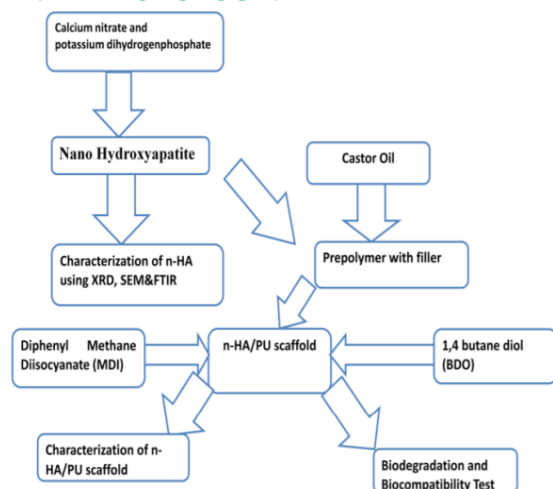
Fig 2: Methodology Flow
