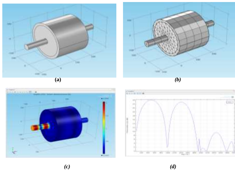
Figure 5: Analysis of Circular Expansion chamber Case II : (a) Modeling (b) Meshing (c) Absolute pressure (d) Transmission loss
