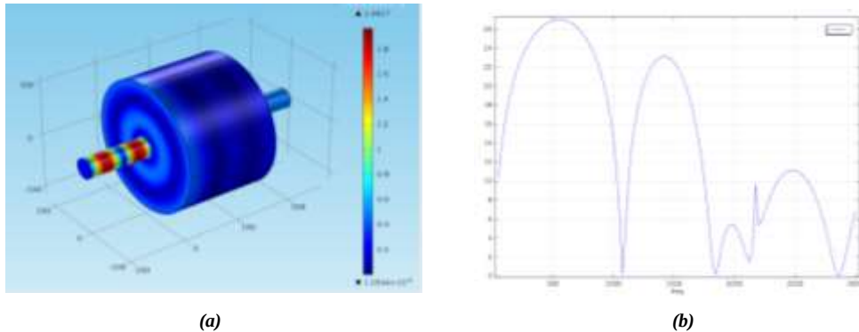
Figure 6: Analysis of Circular Expansion chamber Case IV: (a) Absolute pressure (b) Transmission loss
