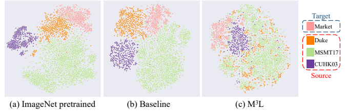
Figure 5: Visual distributions of four person ReID benchmarks. The distributions are obtained from inference features of (a) ImageNet pretrained model, (b) Baseline, and (c) M^3L . All of the models are trained with ResNet-50, and the dimension of inference features is reduced by t-SNE [25].
