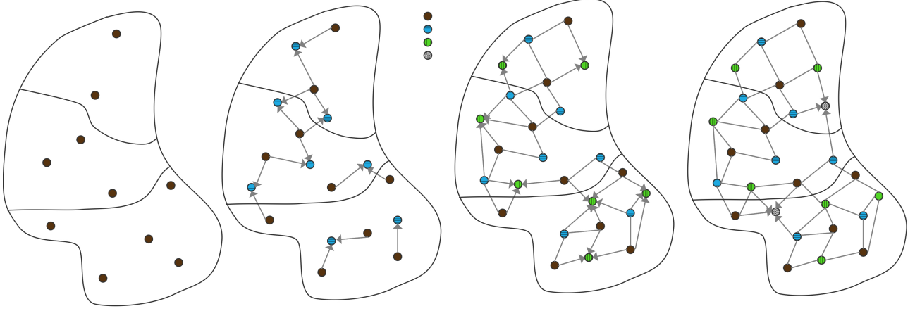
Figure 6.13: Solving a parallel multicolour ILU in four steps
