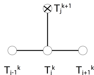
Figure 4.4: The difference stencil of the Euler forward method for the heat equation
