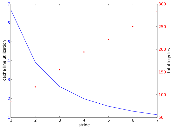
Figure 1.17: Run time in cycles and L1 reuse as a function of stride
