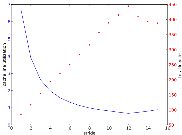
Figure 37.1: Run time in kcycles and L1 reuse as a function of stride
