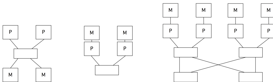
Figure 2.23: A butterfly exchange network for two and four processors/memories
