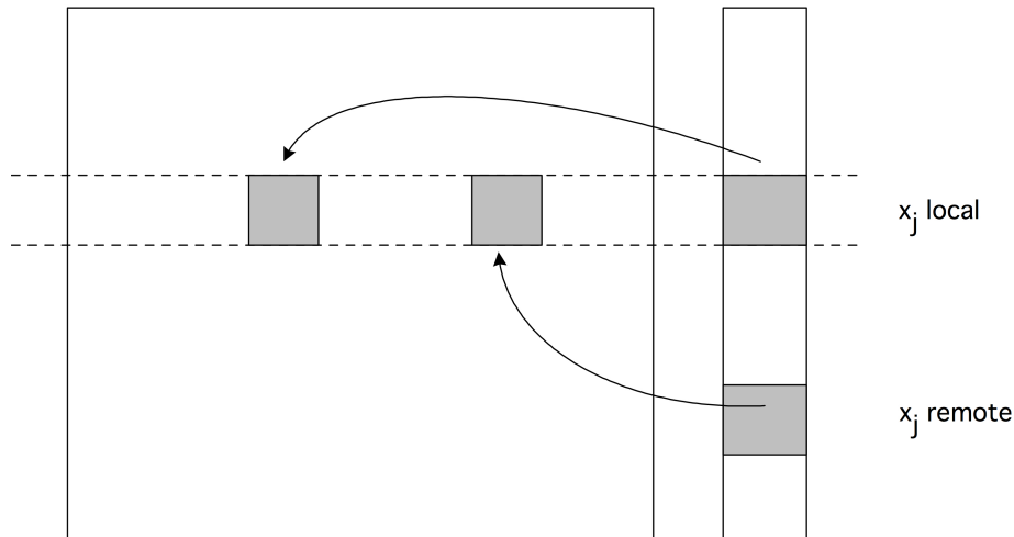
Figure 2.15: The parallel matrix-vector product with a blockrow distribution.
