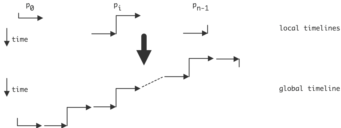
Figure 2.12: Local and resulting global view of an algorithm for sending data to the right
