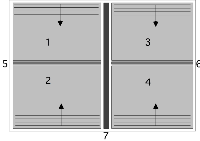
Figure 6.15: A four-way domain decomposition
