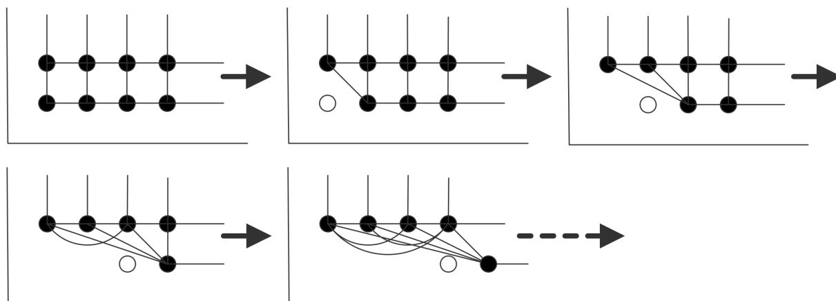
Figure 5.4: Creation of fill-in connection in the matrix graph
