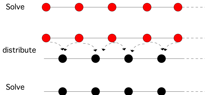
Figure 6.18: Red-black solution on a 1d domain
