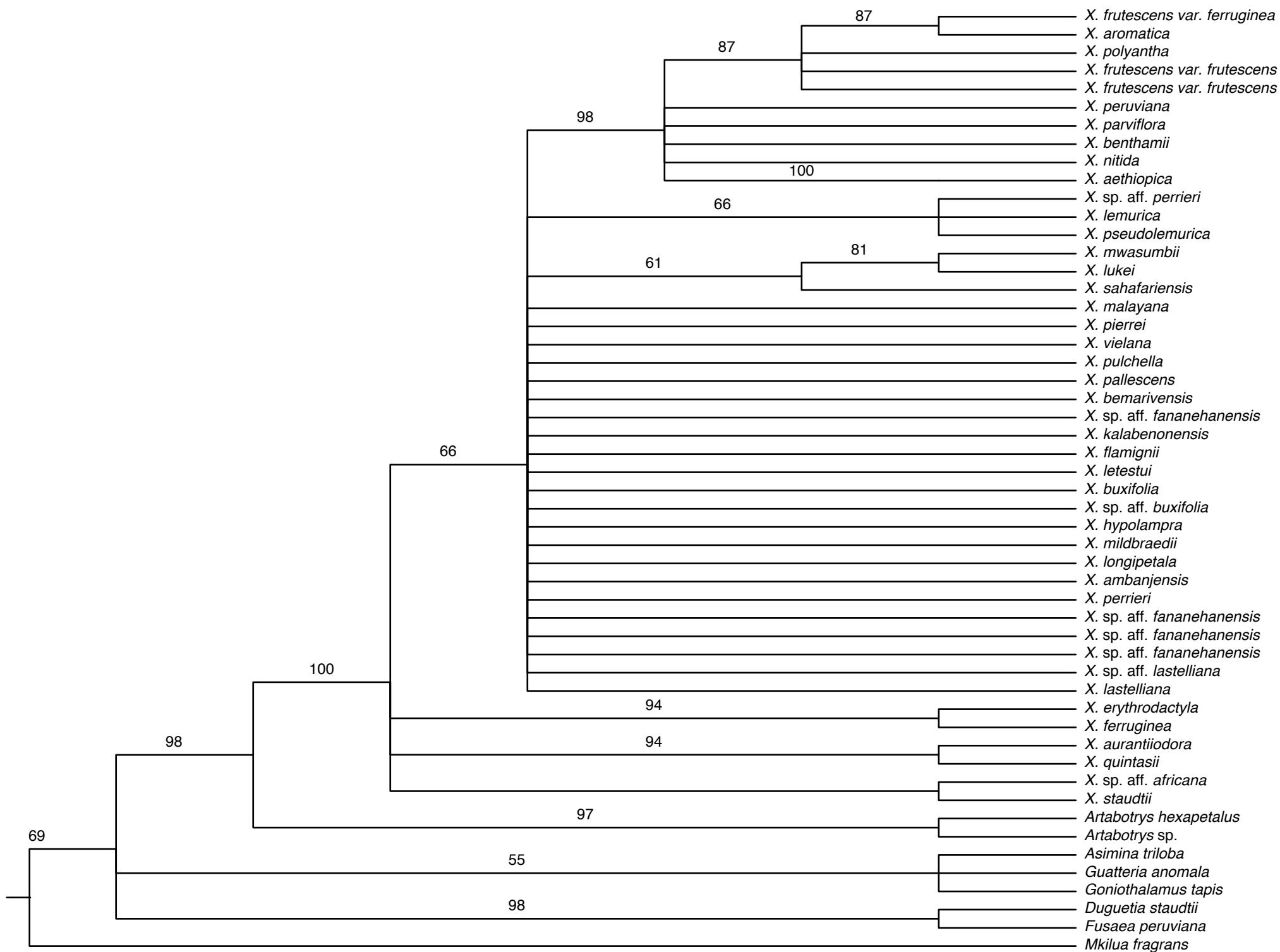
Supplemental Fig. 4. Maximum likelihood analysis of trnL-F spacer, showing bootstrap support.
