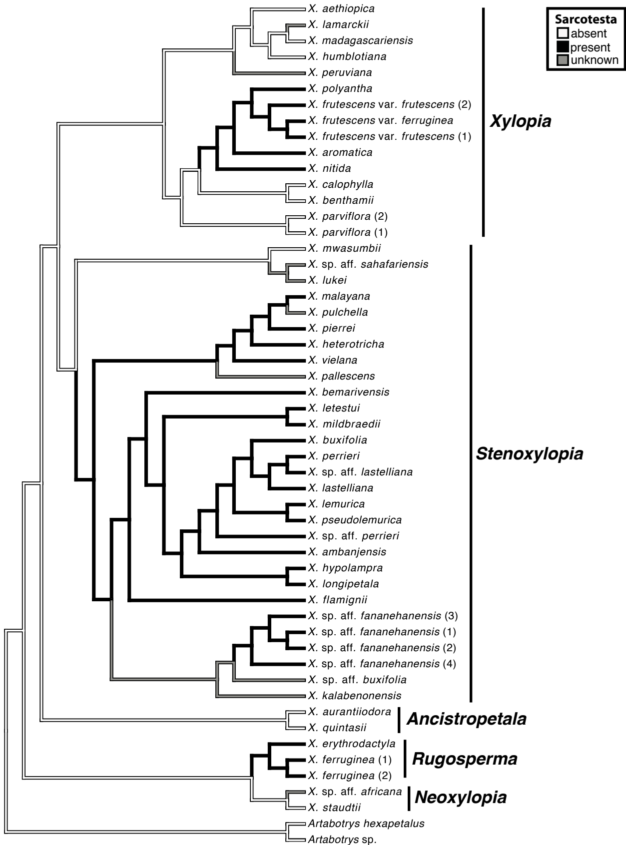
Supplemental Fig. 10. Maximum parsimony reconstruction sarcotesta (presence vs. absence).
