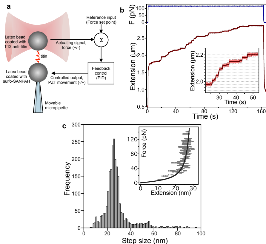
Figure 1. Titin nanomanipulation with force-clamp optical tweezers. a. Experimental layout of the molecular manipulation and feedback control. b. Example of temporal change in the extension of titin in constant force field (115 pN in this example). Force was increased rapidly to
