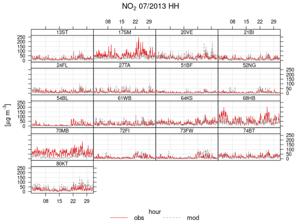
Figure 21: OpenAir time series plots generated by timePlot for observed and modelled data grouped by station.
