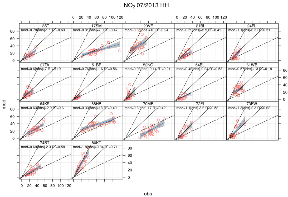
Figure 24: OpenAir scatterplot of (a) monthly averaged data and (b) daily averaged data, grouped by station. The analysis with OpenAir includes all available 17 monitoring stations in Hamburg.
