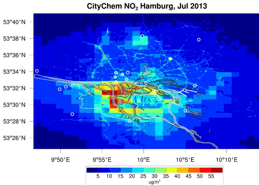
Figure 13: Spatial map of NO 2 monthly concentration average (in \mu\text{g m}^{-3} ) for Hamburg city plotted with the routine create_map.ncl . White outline illustrates harbour areas and black outline illustrates water bodies. Open white circles denote stations.
