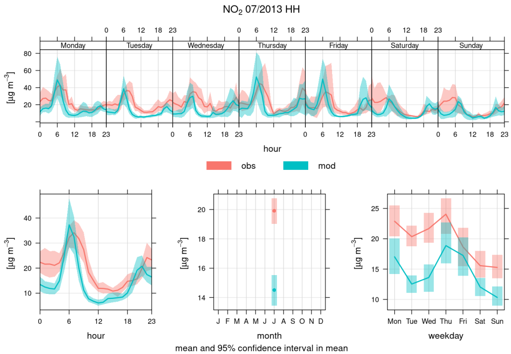
Figure 22: OpenAir temporal variation plots (diurnal and weekly profiles) generated by timeVariation for the modelled and observed data.
