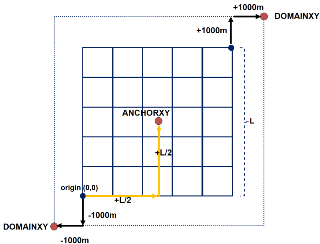
Figure 10: Illustration of the grid definition in AERMAP.
