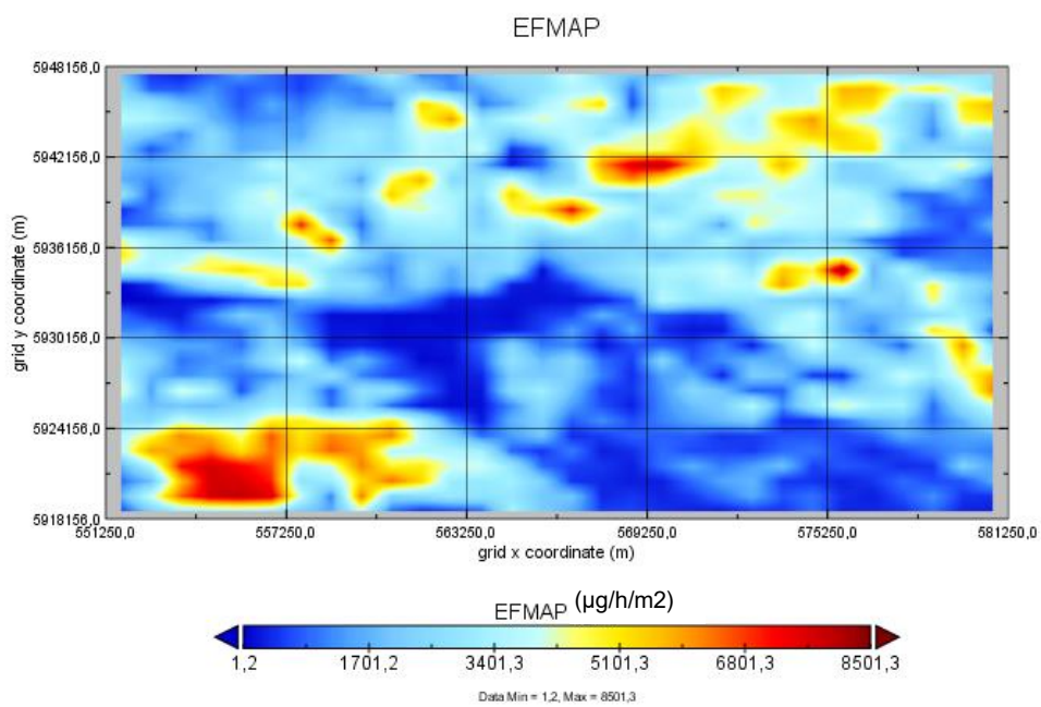
Figure 31: Map of isoprene emission factors for the region of Hamburg: a) isoprene standard emission potential (unit: \mu\text{g}/\text{g}/\text{hr} ) map created based on Copernicus Tree Cover Density and Corine Land Cover; resolution of 100 m; b) interpolated field of emission factor \times foliar density (unit: \mu\text{g}/\text{hr}/\text{m}^2 ) calculated in UECT; resolution of 1000 m in zoom region of a).
