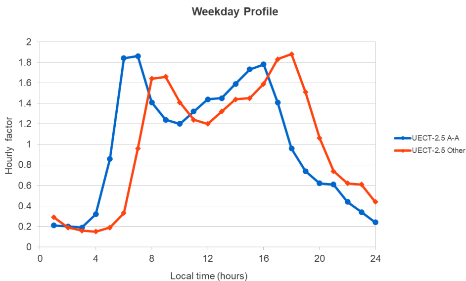
Figure 30: Weekday profile of line source emissions. In UECT v2.3 and later versions, the months April to August are treated with the blue profile. In v2.4 and later versions, the weekday profile for the remaining months of the year are treated with the red profile. In UECT v.2.2 and earlier versions, all months had the same weekday profile.
