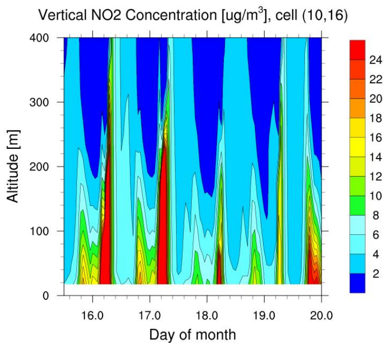
Figure 15: Hourly time slices of the vertical profile of NO 2 mixing ratio (in \mu\text{g m}^{-3} ) for main grid cell (10,16) for 4.5 days in July 2013 (starting at noon of 15 th July) as contour plot created by routine vertical_profile.ncl .
