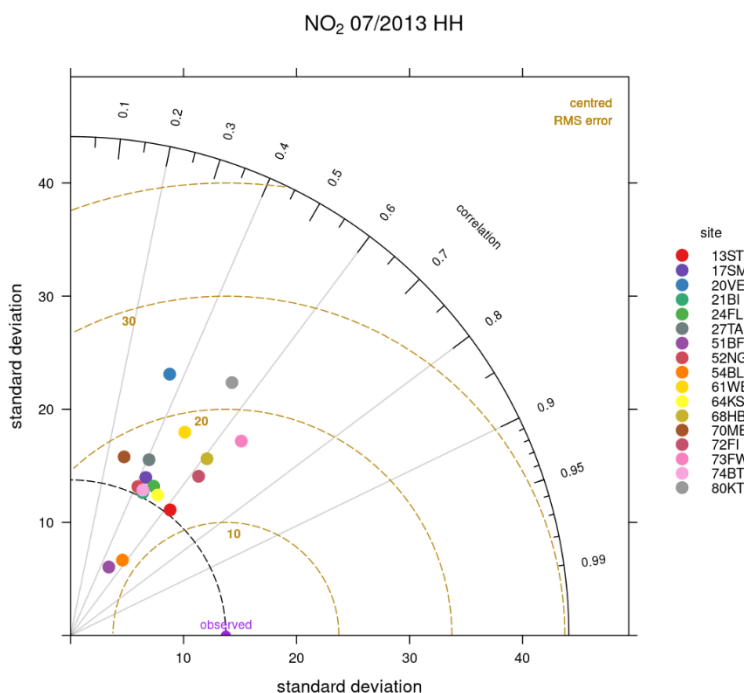
Figure 23: OpenAir generated Taylor diagram of observed and modelled data, grouped by stations.
