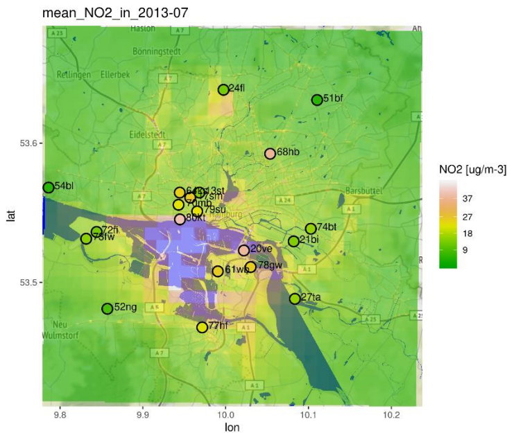
Figure 26: Spatial map of \text{NO}_2 monthly concentration average (in \mu\text{g m}^{-3} ) for Hamburg city plotted with the routine create_ggmap.R . Open black circles denote stations. Blue areas in the background display port areas and water bodies, which are derived from Urban Atlas.
