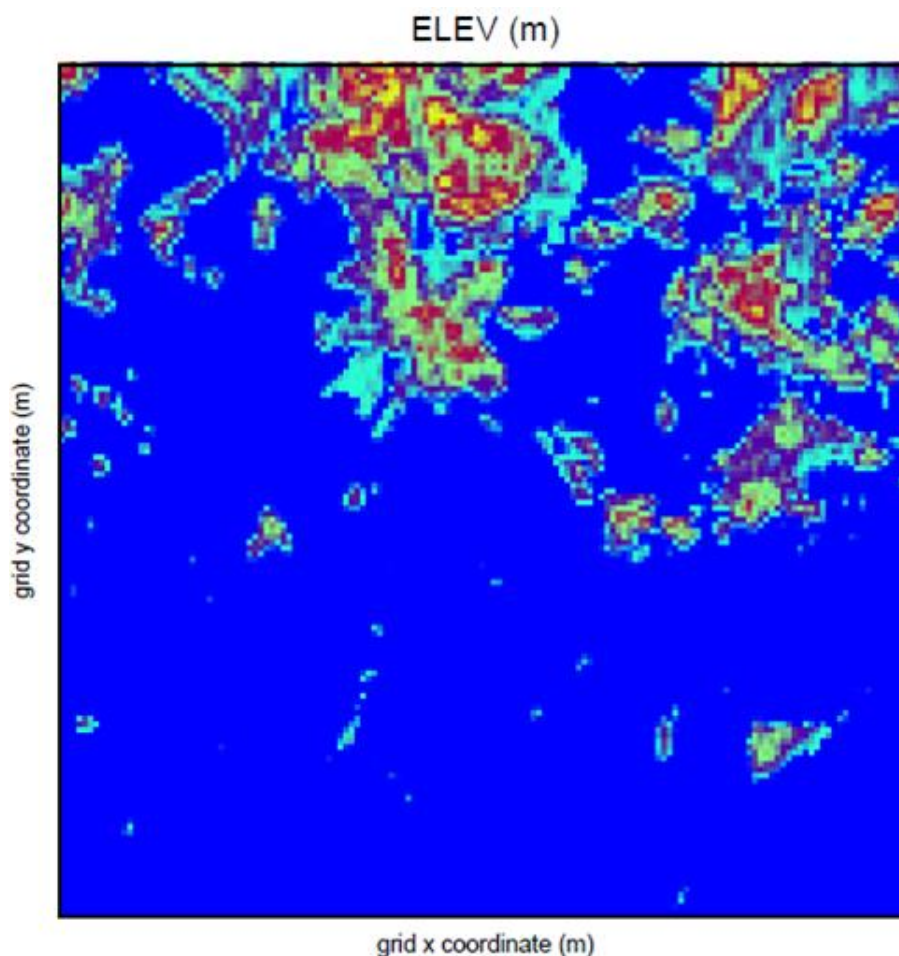
Figure 11: Terrain elevation map (heights in m) of the Helsinki bay with a grid resolution of 100 m, produced from SRTM3 data using the AERMAP terrain pre-processor. Blue colour is sea surface, yellow to red colours show elevations up to 50.9 m.
