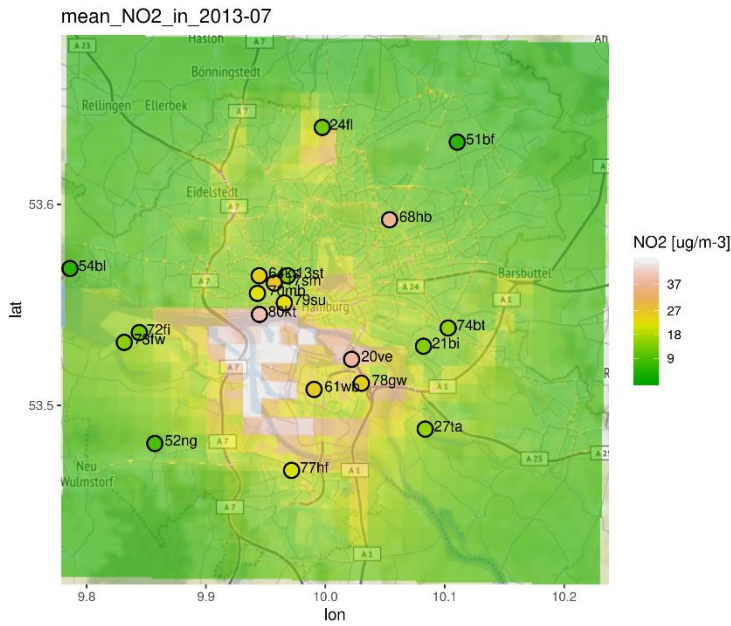
Figure 25: Spatial map of \text{NO}_2 monthly concentration average (in \mu\text{g m}^{-3} ) for Hamburg city plotted with the routine create_ggmap.R . Open black circles denote stations.
