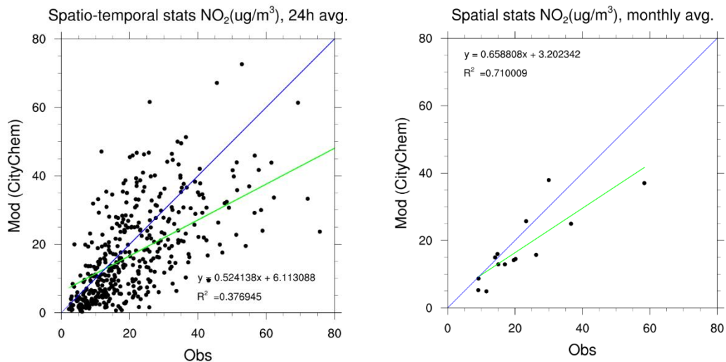
Figure 20: Regression plots of modelled NO 2 concentration versus monitored NO 2 concentration when including 14 monitoring stations in Hamburg using (a) 24-hour averages and (b) monthly averages. Blue line denotes the 1:1 line and the green line is the regression line. Regression parameters are included in the plots.
