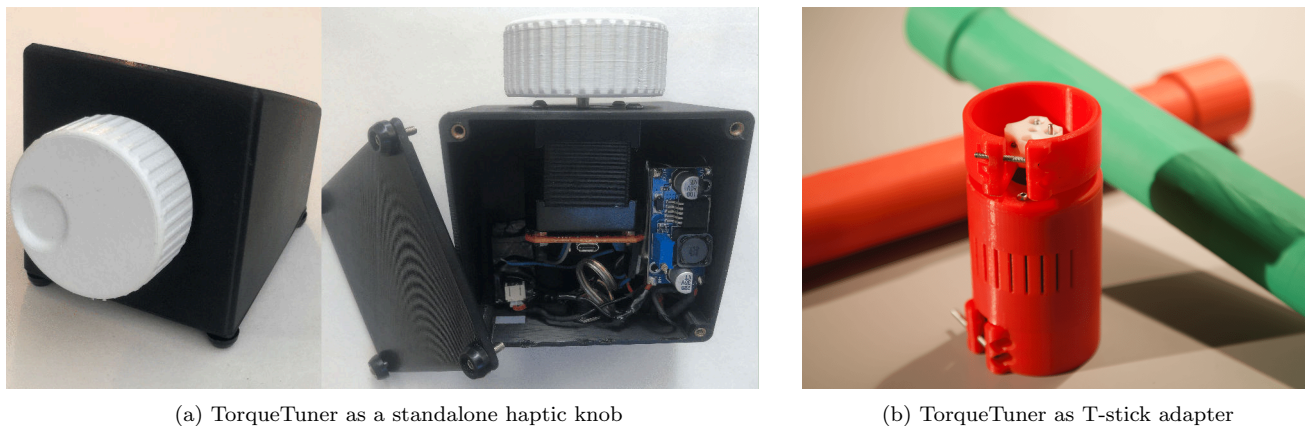
Figure 5: Two examples of modular integrations of TorqueTuner in DMIs
