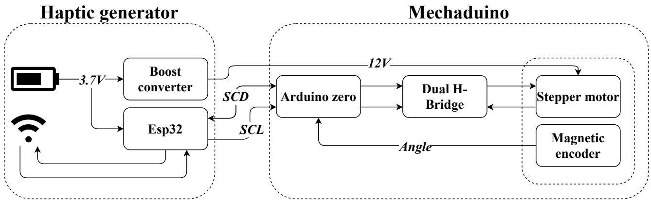
Figure 2: Block diagram of TorqueTuner hardware platform
