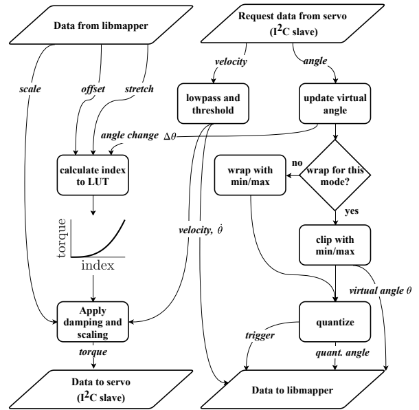
Figure 4: Diagram showing the data flow and -processing of the main update function of the Haptic Generator
