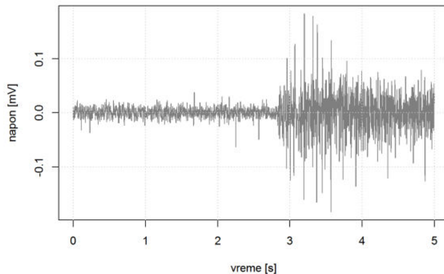
EMG signal
