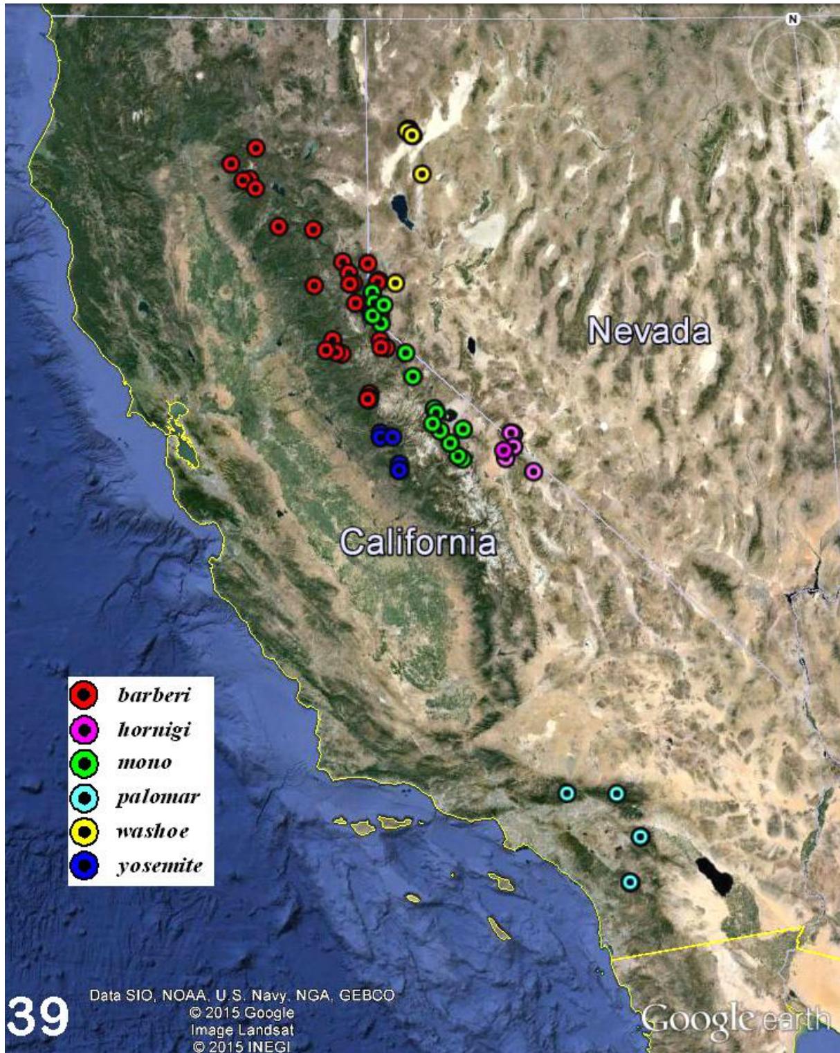
Fig. 39. Distributional map of Sierracapnia spp.: barberi (red), hornigi (purple), mono (dark green), palomar (light blue), washoe (yellow), and yosemite (dark blue).
