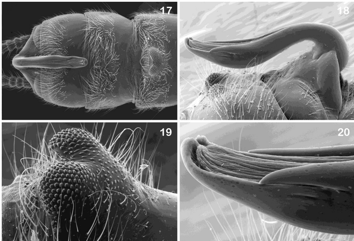
Figs. 17-20. Sierracapnia shepardii . Male: 17. Parker Creek, California. Genitalia, dorsal, epiproct and knob on tergum 7. 18. South Fork Yuba River, California. Genitalia, lateral, epiproct and knobs on tergum 9. 19. Parker Creek, California. Knob on tergum 7, dorsolateral. 20. South Fork Yuba River, California. Epiproct, lateral, apex.
