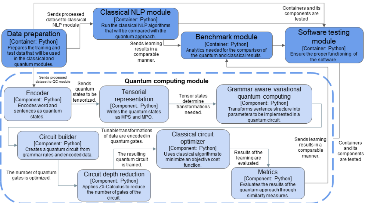
Figure 7. Component-level diagram of quantum NLP module.
