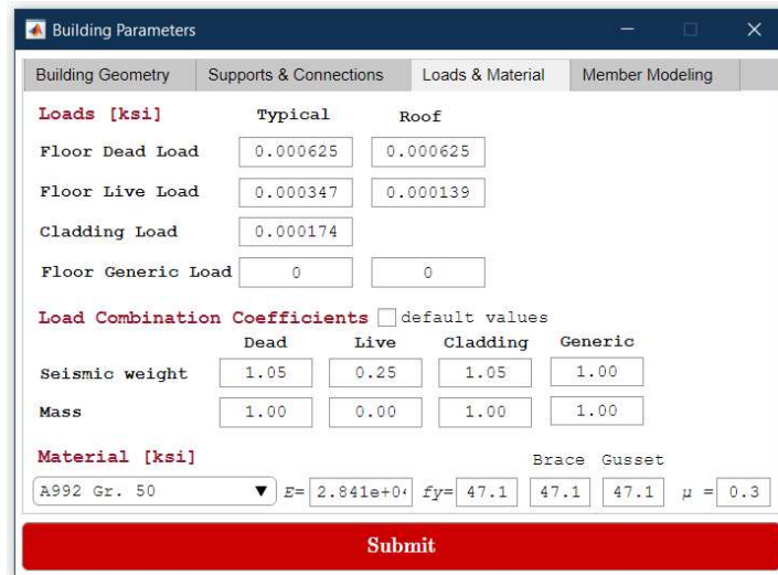
Figure 4.11. Building parameters module: Loads and material tab
