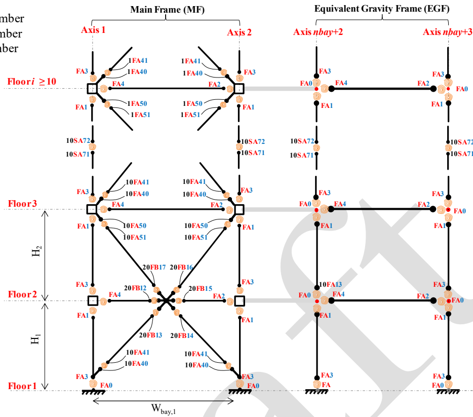
(a) Node notation
