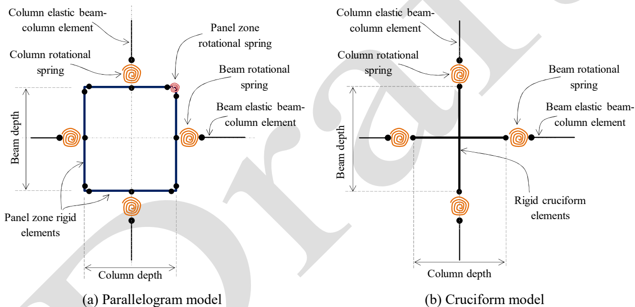
Figure 7.2. Types of panel zone idealization when (a) considered and (b) ignored
