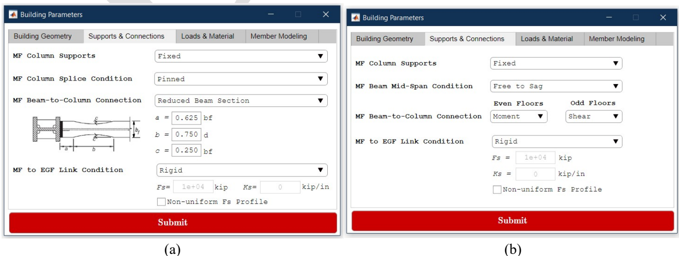
Figure 4.9. Building parameters module: Supports and connections tab for (a) MRF and (b) CBF
