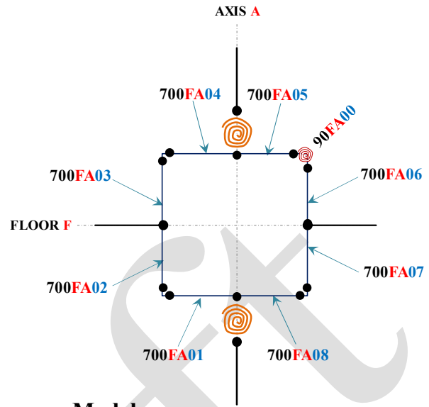
Parallelogram Model
