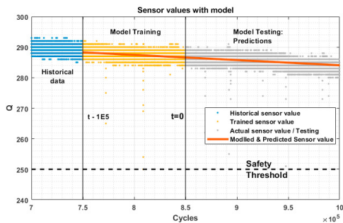
Fig. 7. f(t) model between cycles 7.5 \times 10^5 to 8.5 \times 10^5 (current) with the estimated parameter of \phi(t) = -1.689 \times 10^{-5} and \sigma = 300.9 .
