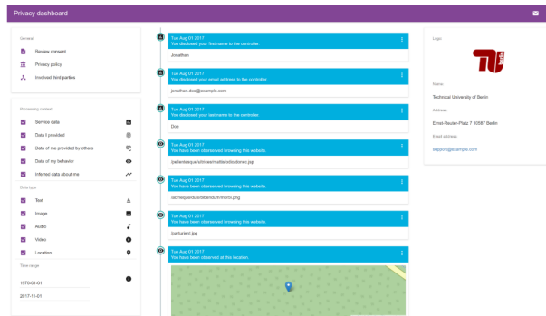
Fig. 3. The GDPR-compliant and Usable Privacy Dashboard by Rashcke et al. [33]
