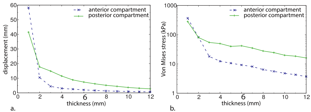
Fig. 3. The effect of varying thickness and constant surface area ( R = 1 ) and pressure (4 kPa) on (a) pelvic floor displacement and (b) Von Mises stress. For thicknesses of 1 to 3 mm, the pelvic floor deflected most strongly (up to 60 mm), whereas beyond a thickness of 3 mm, displacement decreased more gradually (a). Similar behavior was observed for stresses (b). The range of 1 to 12 mm roughly corresponds to the variation in thickness across the pelvic floor and among individuals reported in the literature (SI Appendix, Table S1). The thickness of the base model is 6 mm.
