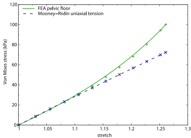
Fig. 5. Stress–stretch behavior of the pelvic floor finite element model with average dimensions (green) compared with the analytical Mooney–Rivlin relations for uniaxial tension using material parameters based on continent women (blue dashed). The model was subjected to a pressure of 15 kPa. The stress–stretch relationship in the FE model clearly deviates from the uniaxial linear response and shows a nonlinear relation for a stretch higher than 1.11 and a corresponding Von Mises stress higher than 30 kPa.
