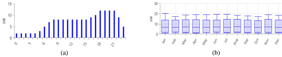
Figure 2. Electric load.
