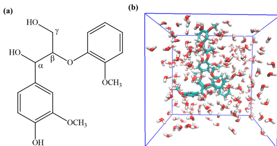
Figure 1. (a) Lignin model—Guaiacyl glycerol-β-guaiacyl ether (GGE) (b) The simulation box contains three GGE and 200 water molecules.
