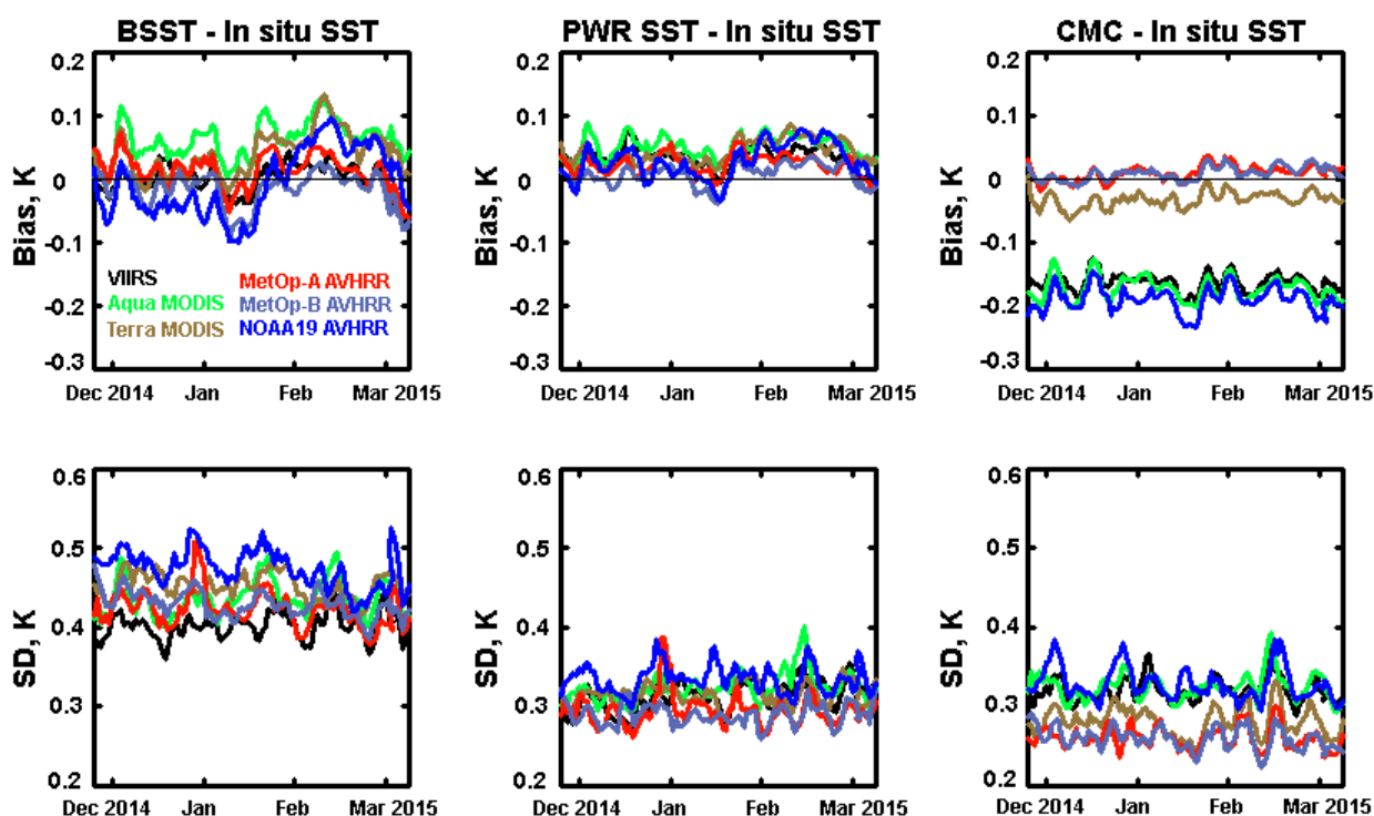
Fig. 2. Daytime time series of daily global biases and SDs of fitting in situ SST with BSST, PWR SST and CMC, for six satellite sensors, from 24 November 2014 to 10 March 2015.
