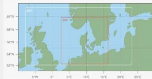
Figure 12: WRF domain set-up
