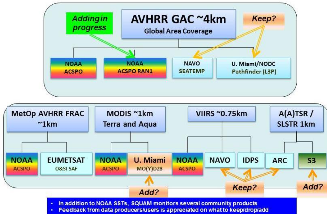
Figure 1: Data currently monitored in SQUAM. Top: low resolution (~4km); Bottom: high resolution data (~1km).
