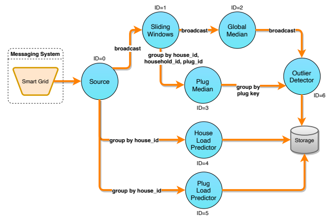
FIGURE 15: Smart Grid Monitoring application (SM).
