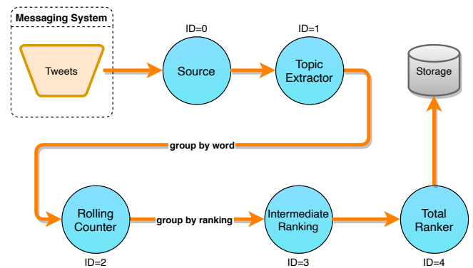
FIGURE 9: Trending Topic application (TT).
