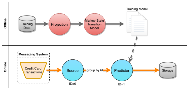
FIGURE 11: Fraud Detection application (FD).
