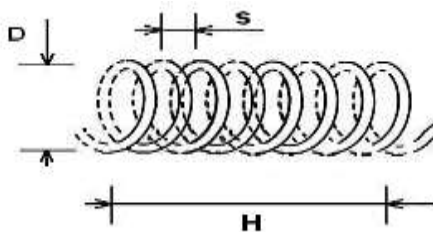
Fig.3 Helical shape.
