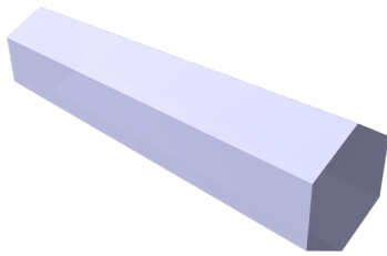
Figure 1.1. Shape rendering.
