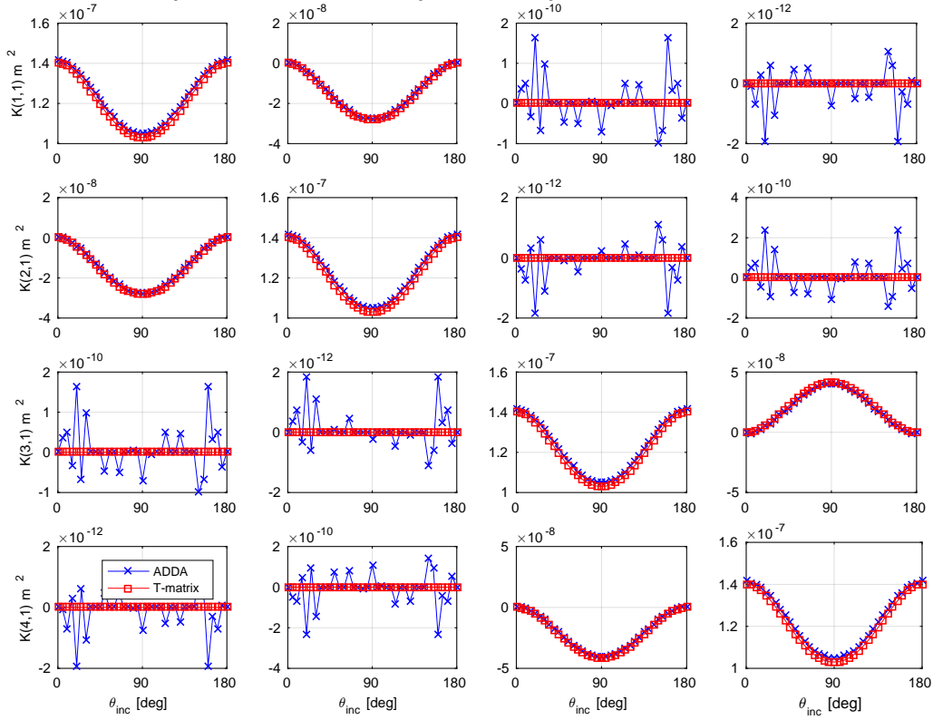
Extinction matrix --- ellipsoid_1.0_2.00_0-90-0_deq00521um_freq183.0GHz_T0253K --- AR=0.5
