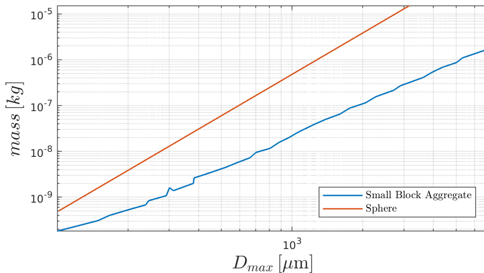
Figure 1.2. Mass-size relationship
