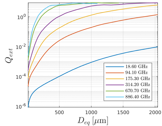
Figure 2.1. Extinction
