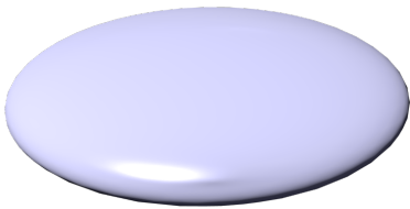
Figure 1.1. Shape rendering.
