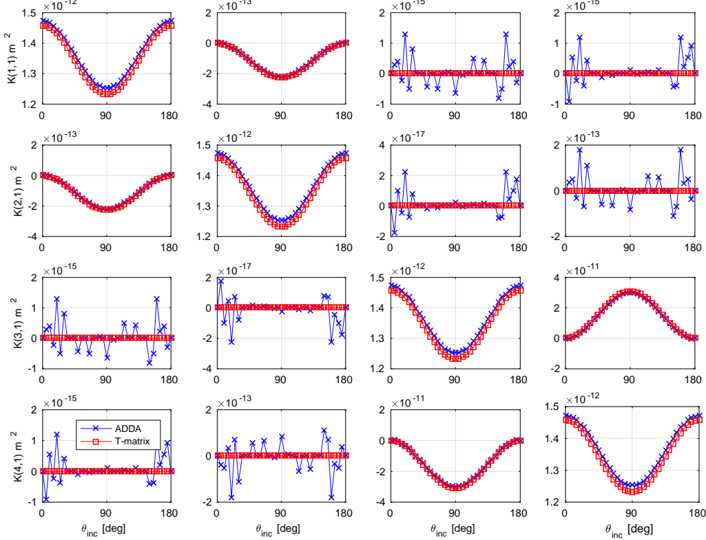
Extinction matrix --- ellipsoid_1.0_2.00_0-90-0_deq00052um_freq183.0GHz_T0253K --- AR=0.5
