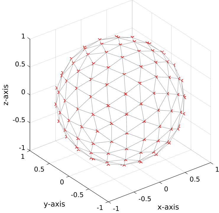
Figure 4.1.: Example of an icosphere grid with 162 vertices. Each gridpoint represent an incoming angle for which a DDA calculation is preformed. This type of configuration ensures that the grid density is isotropic, making the overall calculations more efficient (a standard polar grid would be inefficient since it yields an excessive amount of angles around the ‘North and South poles’’).
