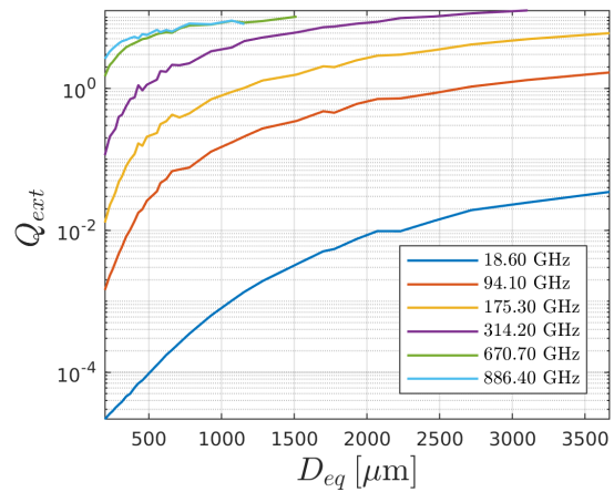
Figure 2.1. Extinction
