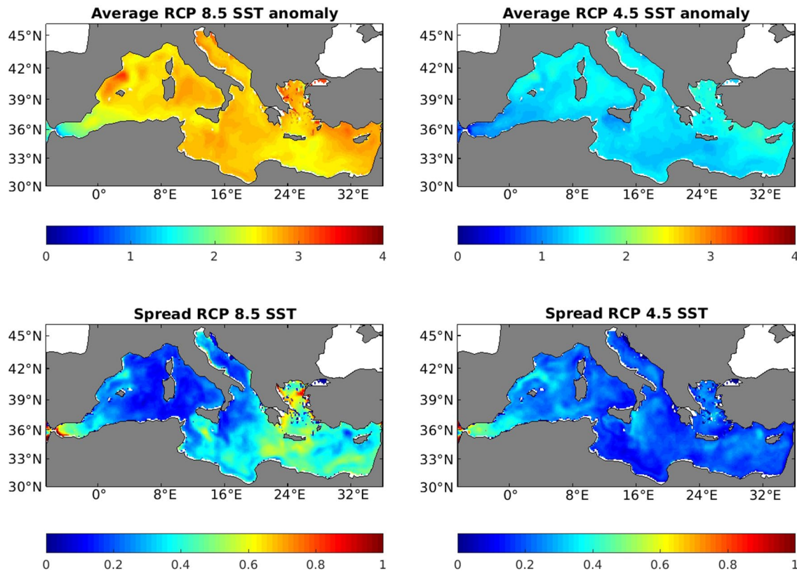
Fig. 3 Average SST anomalies ( ^{\circ}\text{C} ) for the RCP 8.5 runs (top left) and RCP 4.5 runs (top right). The bottom left and right panels are the spread of the RCP 8.5 and RCP 4.5 sub-ensembles, respectively
