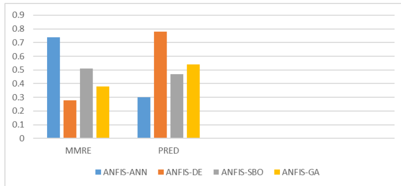
Figure 1. PRED and MMRE criteria values plot in Albrecht dataset
