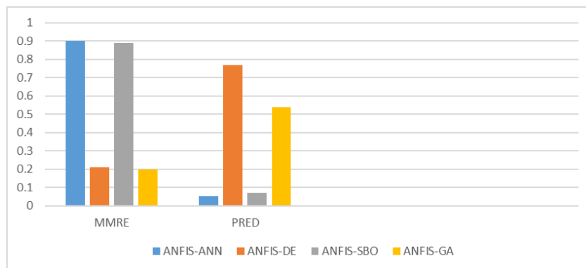
Figure 2. PRED and MMRE criteria values plot in Kemerer dataset
