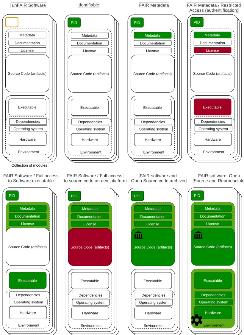
Figure 1. Summarizing software as increasingly FAIR research objects (Credit: Morane Gruenpeter, inspired by the FORCE11 diagram 2 )
