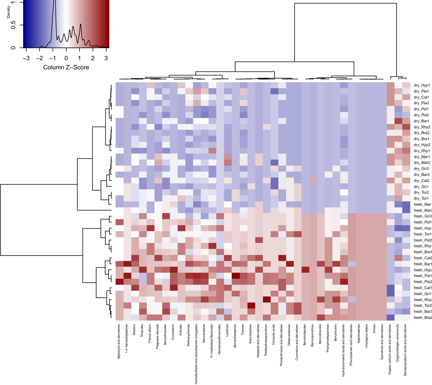
sPLS-DA
