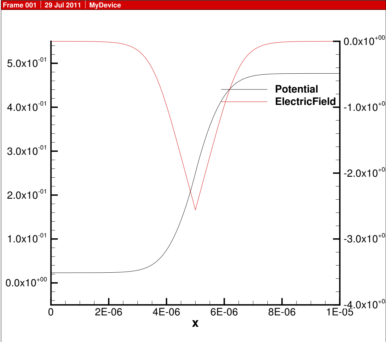
Fig. 17.2: Potential and electric field versus position in 1D diode.
