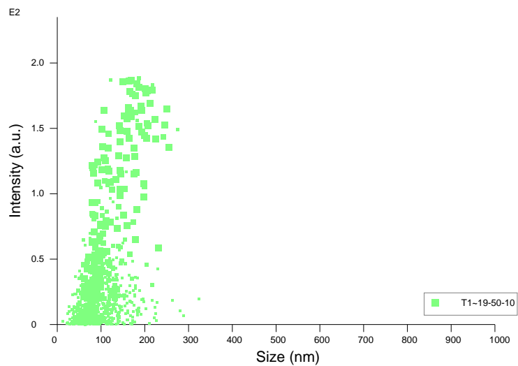
Intensity / Size graph for Experiment: T1 2020-02-21 19-49-57
