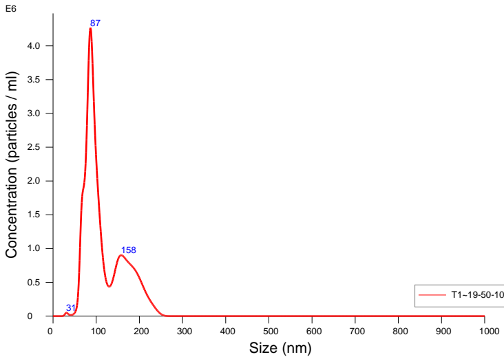
FTLA Concentration / Size graph for Experiment: T1 2020-02-21 19-49-57
