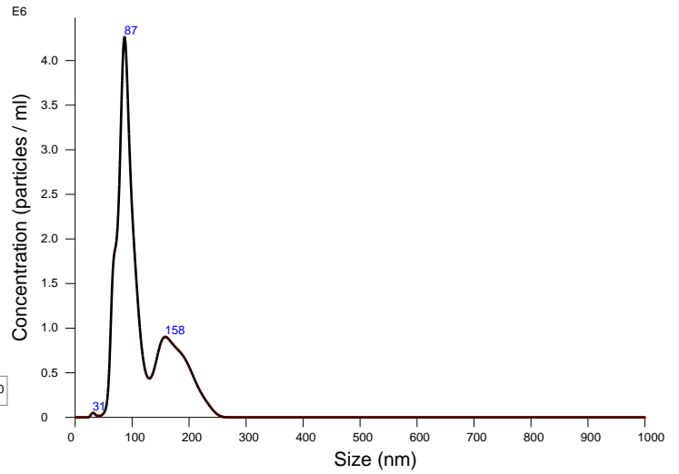
Averaged FTLA Concentration / Size for Experiment: T1 2020-02-21 19-49-57 Error bars indicate + / -1 standard error of the mean
