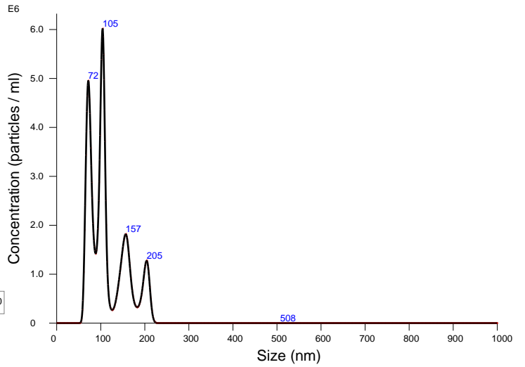
Averaged FTLA Concentration / Size for Experiment: MSC2 2020-02-21 18-48-59 Error bars indicate + / -1 standard error of the mean
