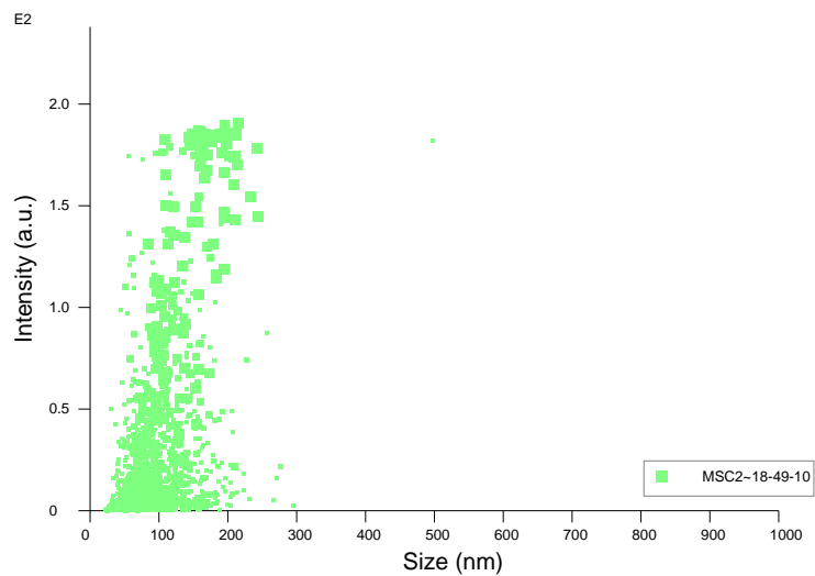
Intensity / Size graph for Experiment: MSC2 2020-02-21 18-48-59
