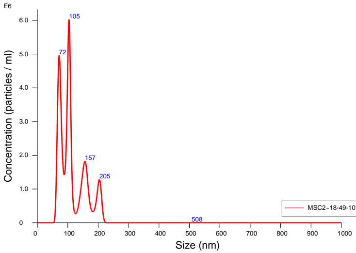
FTLA Concentration / Size graph for Experiment: MSC2 2020-02-21 18-48-59
