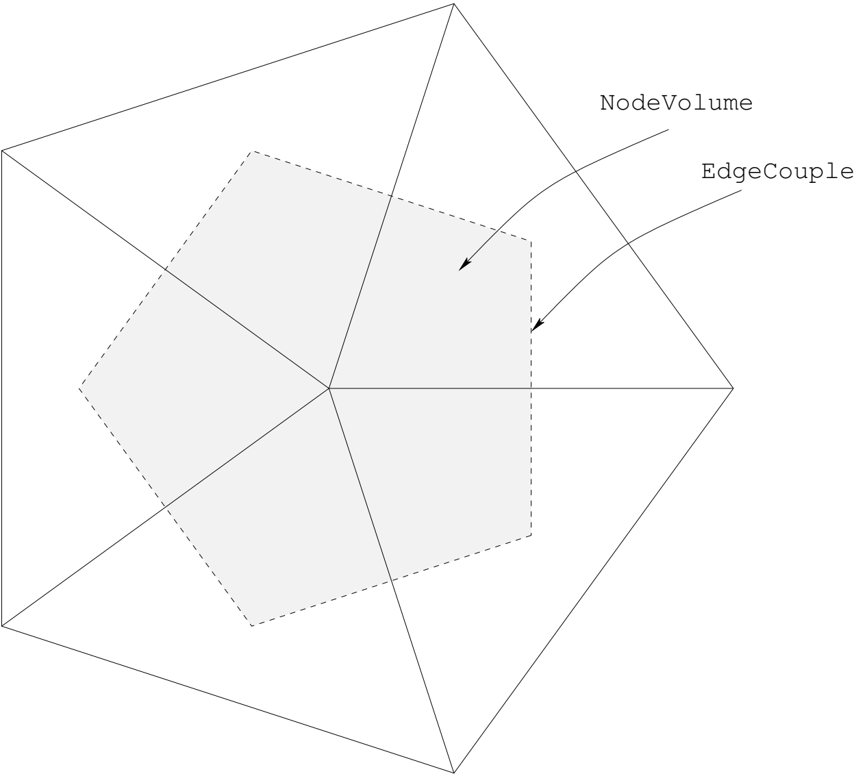
Fig. 4.1: Mesh elements in 2D.
