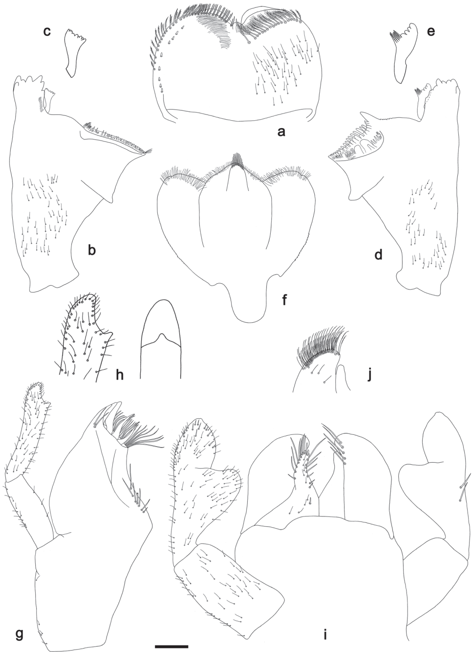
Figure 5. Labiobaetis excavatus sp. nov., nymph morphology: a labrum b right mandible c right prostheta d left mandible e left prostheta f hypopharynx and superlinguae g maxilla h apex of maxillary palp (left: dorsal view, right: inner lateral view) i labium j apex of paraglossa. Scale bar: 0.1 mm.
