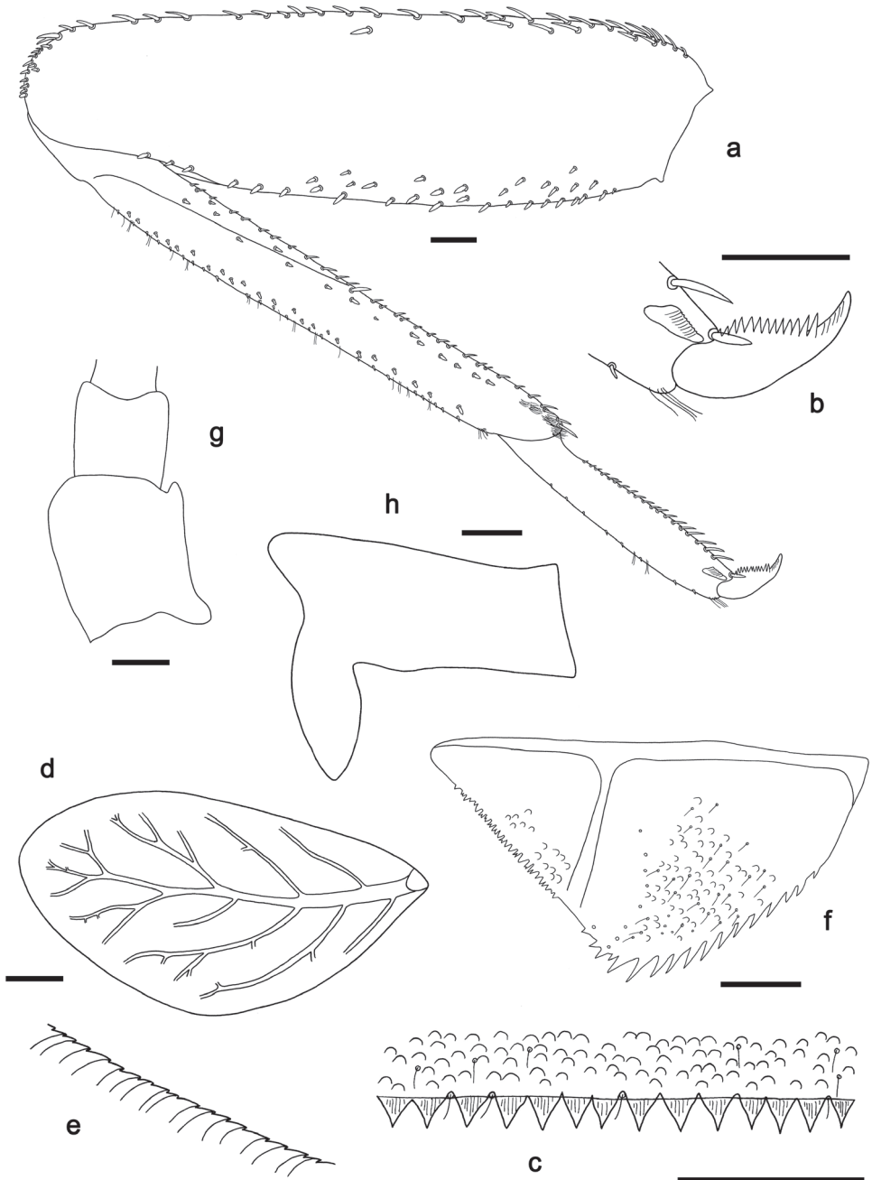
Figure 4. Labiobaetis excavatus sp. nov., nymph morphology a foreleg b fore claw c tergum IV d gill IV e margin of gill IV f paraproct g antennal scape h metanotum. Scale bars: 0.1 mm.
