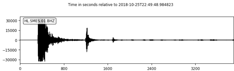
Figure 8: Seismogram in Logga
