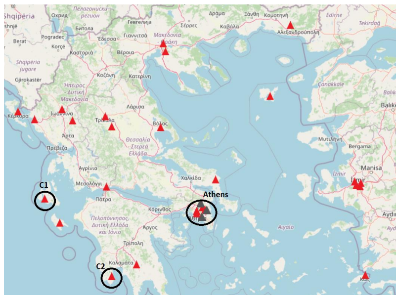
Figure 6: Map, C 1 first stimulated seismograph in Argostoli, C 2 second stimulated seismograph in Logga, target: Athens
