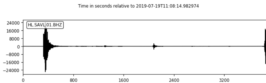
Figure 13: Seismogram in Avlonari
