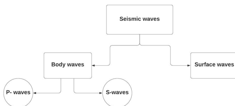
Figure 2: Different kinds of seismic waves
