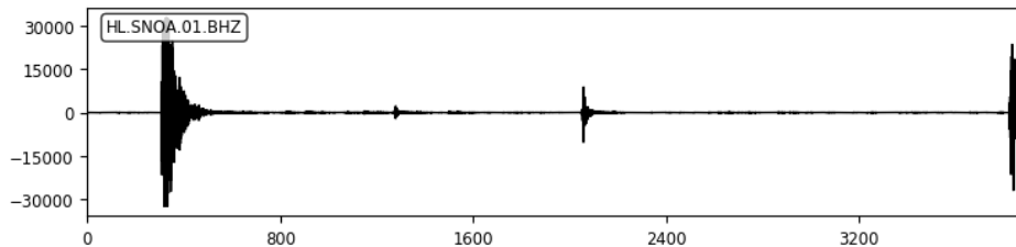
Figure 11: Seismogram in the Geodynamic Institute of Athens
