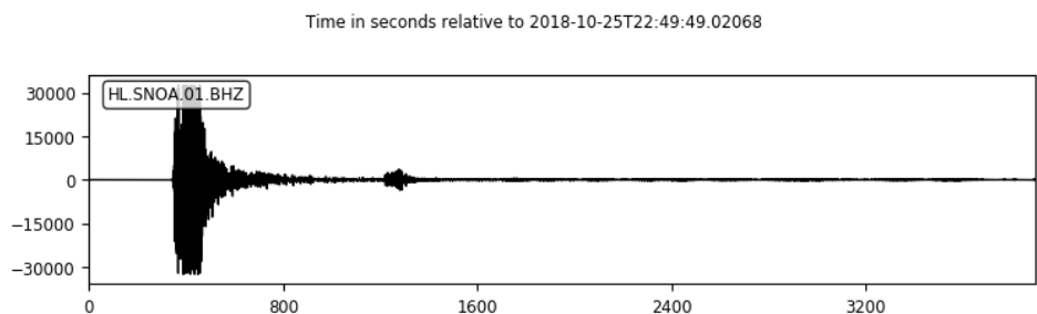
Figure 9: Seismogram in the Geodynamic Institute of Athens
