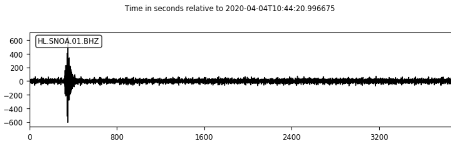
Figure 16: Seismograph in the Geodynamic Institute of Athens
