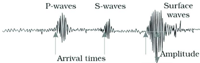
Figure 3: Seismic waves in a seismograph
