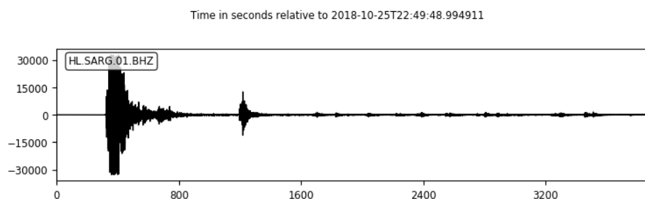
Figure 7: Seismogram in Argostoli
