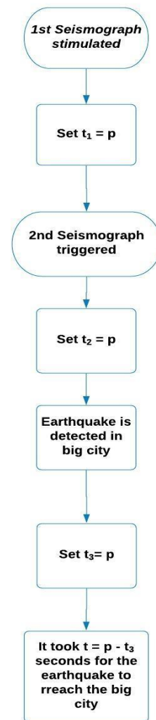
Figure 5: Time differences chart
