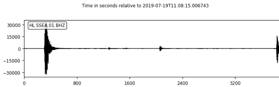
Figure 12 Seismogram in Pallini
