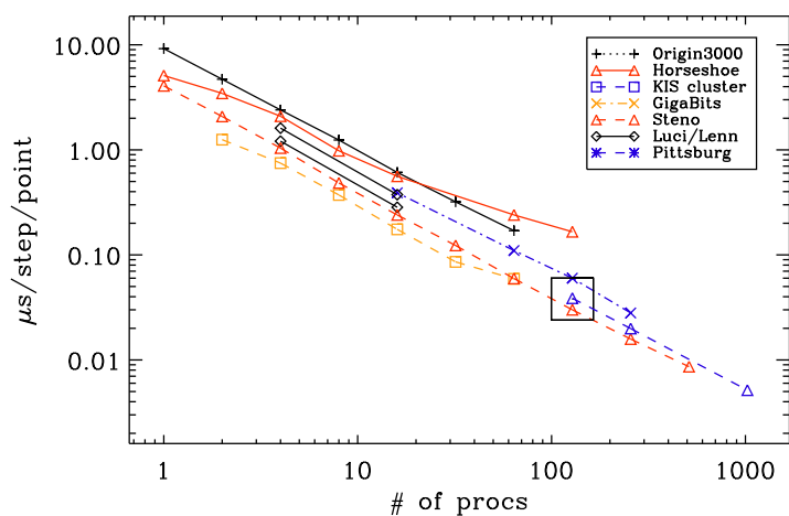
Figure 13: Scaling results on three different machines. The thin straight line denotes perfectly linear scaling.
