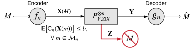
Fig. 1. The CC WTC with transition kernel P_{Y,Z|X} . The encoder outputs \mathbf{X}(m) for message M = m , and the decoder and the eavesdropper observes \mathbf{Y} and \mathbf{Z} , respectively. The cost constraint \mathbb{E}[C_n(\mathbf{X}(m))] \leq b is imposed for each message m \in \mathcal{M}_n .
