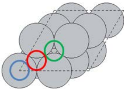
Metal FCC (111) Surface
