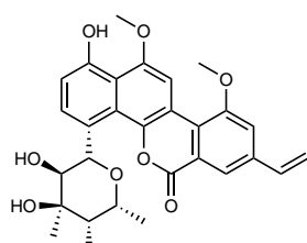
Chrysomycin A
