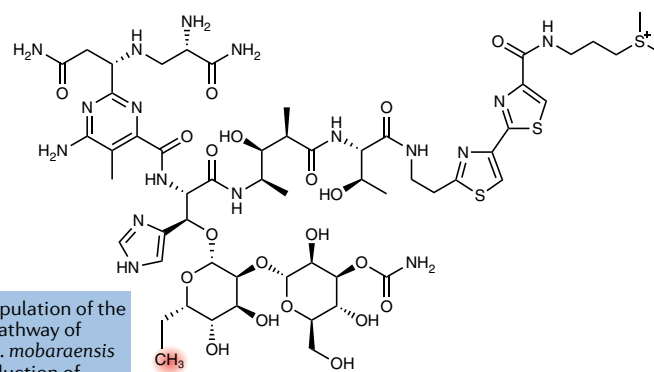
6'-deoxy-BLM A2
