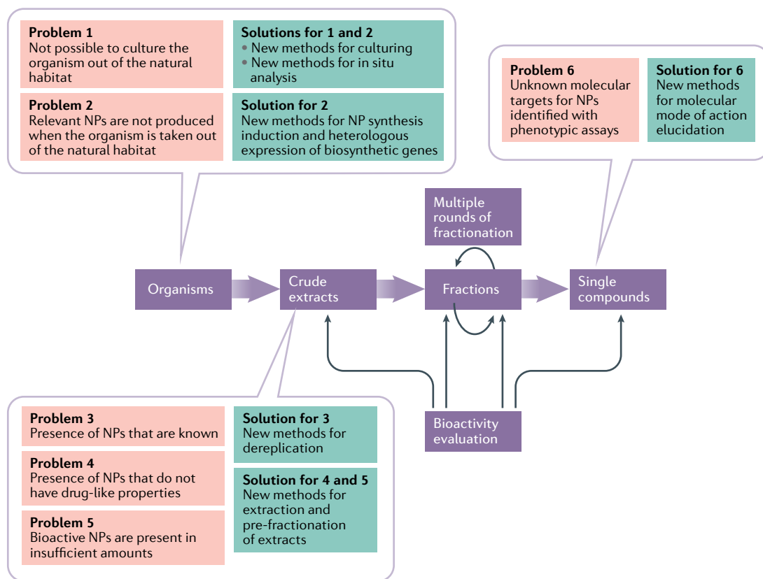
Fig. 1 | Outline of traditional bioactivity-guided isolation steps in natural product drug discovery. Steps in the process are shown in purple boxes, with associated key limitations shown in red boxes and advances that are helping to address these limitations in modern natural product (NP)-based drug discovery shown in green boxes. The process begins with extraction of NPs from organisms such as bacteria. The choice of extraction method determines which compound classes will be present in the extract (for example, the use of more polar solvents will result in a higher abundance of polar compounds in the crude extract). To maximize the diversity of the extracted NPs, the biological material can be subjected to extraction with several solvents of different polarity. Following the identification of a crude extract with promising pharmacological activity, the next step is its (often multiple) consecutive bioactivity-guided fractionation until the pure bioactive compounds are isolated. A key limitation for the potential of this approach to identify novel NPs is that many potential source organisms cannot be cultured or stop producing relevant NPs when taken out of their natural habitat. These limitations are being addressed through development of new methods for culturing, for in situ analysis, for NP synthesis induction and for heterologous expression of biosynthetic genes. At the crude extract step, challenges include the presence in the extracts of NPs that are already known, NPs that do not have drug-like properties or insufficient amounts of NPs for characterization. These challenges can be addressed through the development of methods for dereplication, extraction and pre-fractionation of extracts. Finally, at the last stage, when bioactive compounds are identified by phenotypic assays, significant time and effort are typically needed to identify the affected molecular targets. This challenge can be addressed by the development of methods for accelerated elucidation of molecular modes of action, such as the nematic protein organization technique (NPOT), drug affinity responsive target stability (DARTS), stable isotope labelling with amino acids in cell culture and pulse proteolysis (SILAC-PP), the cellular thermal shift assay (CETSA) and an extension known as thermal proteome profiling (TPP), stability of proteins from rates of oxidation (SPROX), the similarity ensemble approach (SEA) and bioinformatics-based analysis of connectivity (connectivity map, CMAP) 23,189–192 .
