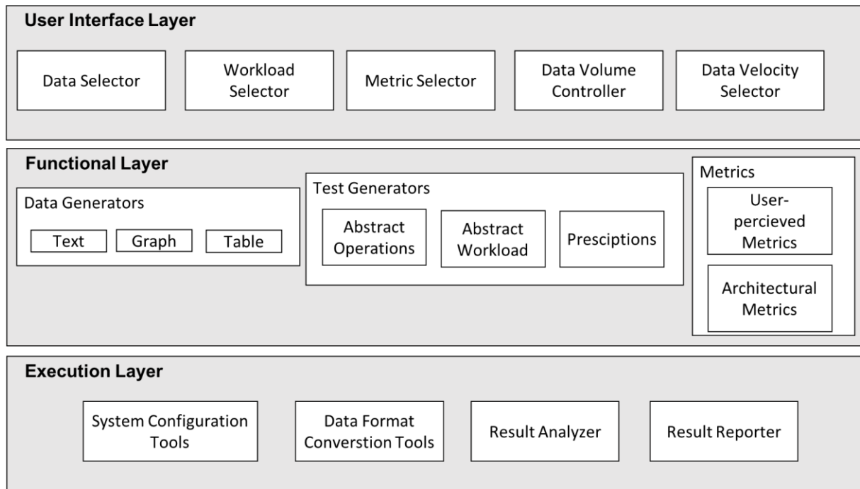
Figure 2: Design Layers of a Big Data Benchmark
