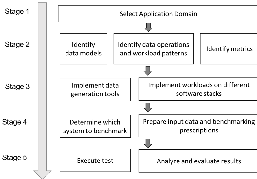
Figure 5: The five-stage benchmarking methodology for a big data system
