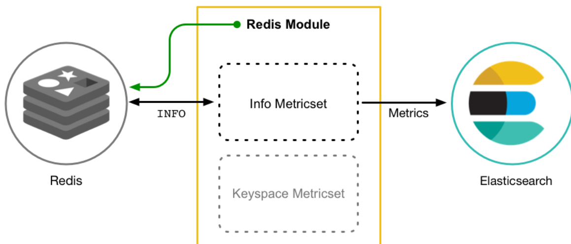
Figure 6: Example of a MetricBeat’s Module
