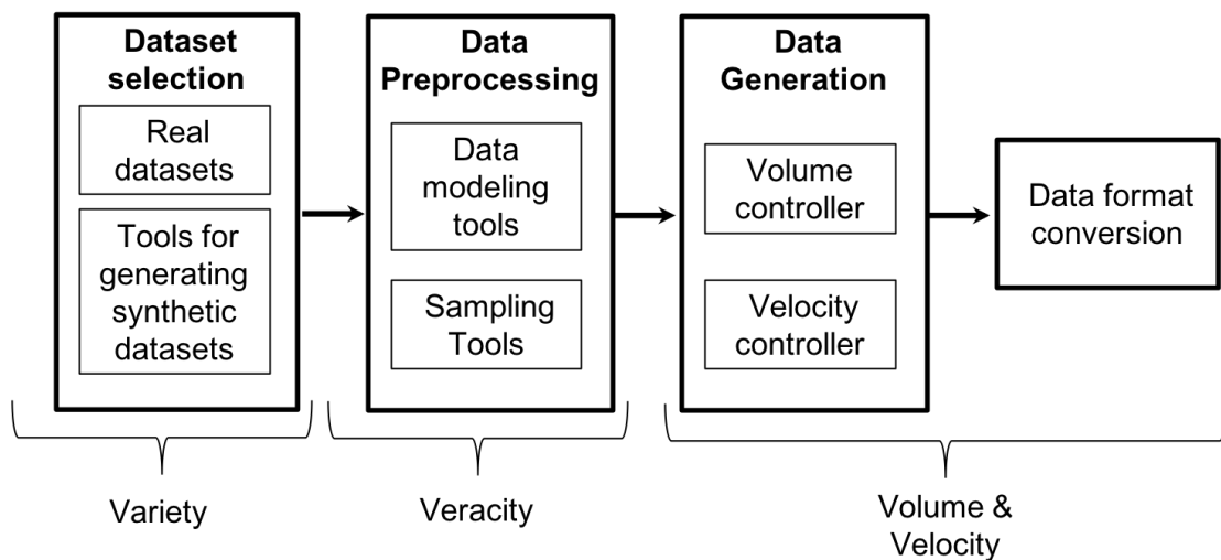
Figure 3: The big data generation process
