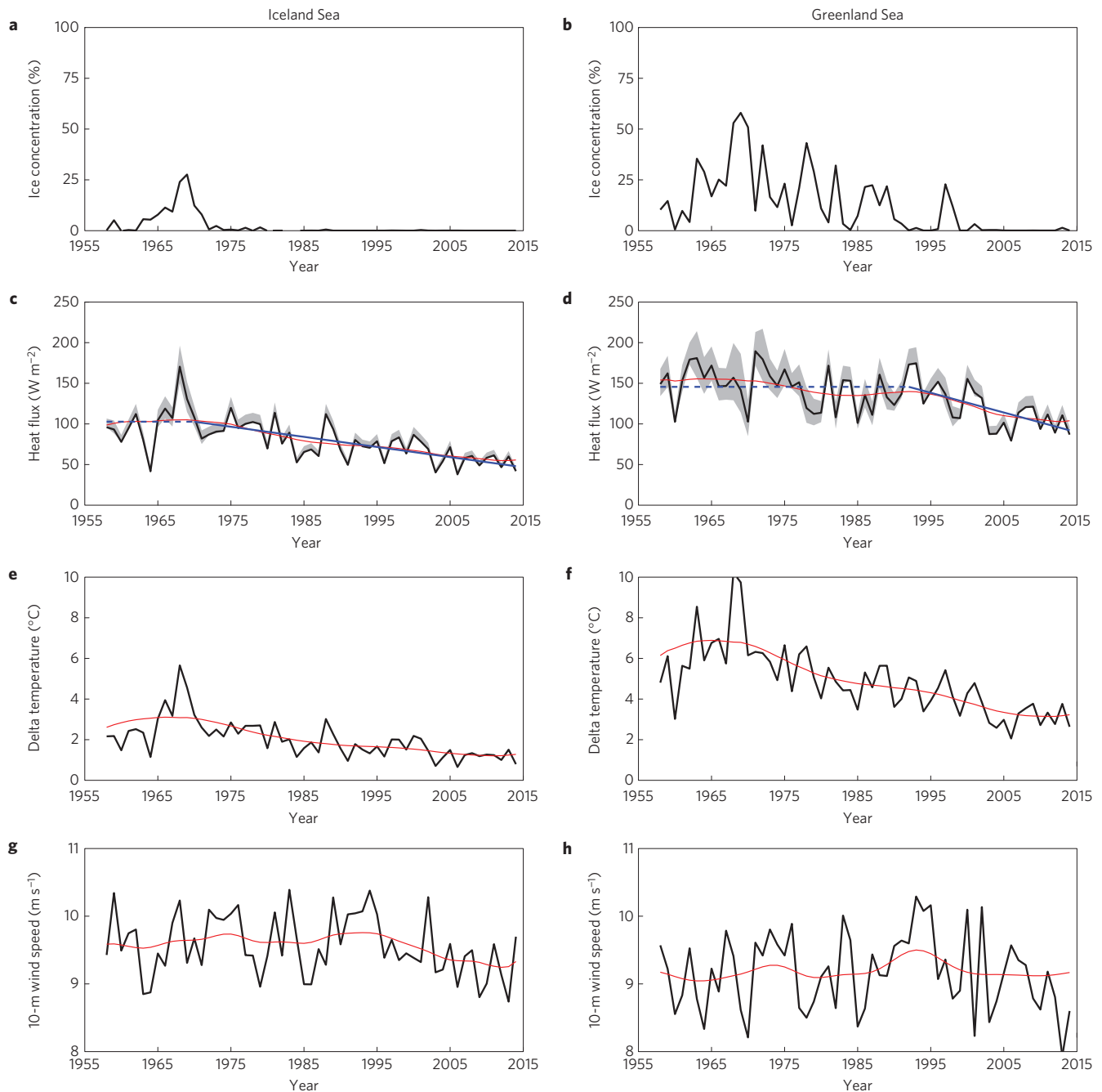
Figure 2 | Time series of the winter-mean conditions over the Iceland and Greenland sea gyres. a,b , Sea-ice concentration. c,d , Open-ocean turbulent heat flux, with the shading representative of the uncertainty associated with the sea-ice concentration. e,f , Air-sea temperature difference. g,h , 10-m wind speed. The red curves are the SSA reconstructions of the low-frequency variability in the time series, whereas the blue dashed lines in c and d are continuous piecewise linear least-squares fits. The trend lines that are solid are statistically significant at the 95% confidence level.
