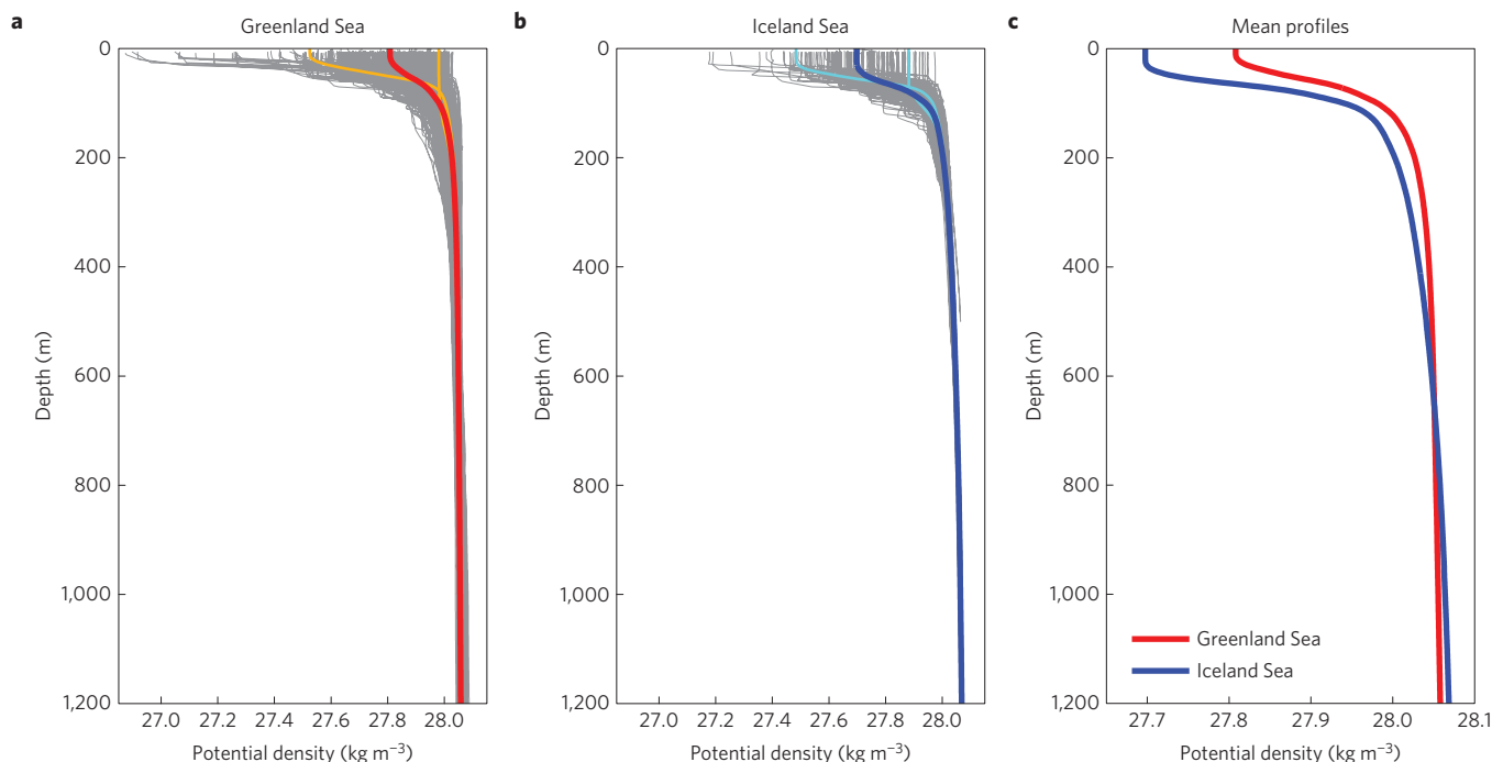
Figure 3 | Potential density profiles for October and November used as initial conditions for the PWP model. a, b , Profiles for the Greenland Sea ( a ) and the Iceland Sea ( b ). The traces are individual profiles (grey), means of the 20% most- and least-stratified profiles (orange and cyan), and overall means (red and blue). c , Comparison of the mean profile from each gyre. Note the different x-axis scale.
