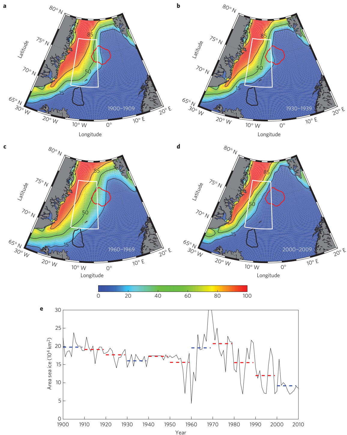
Figure 1 | Winter sea-ice extent for the Nordic seas. a–d , Four decadal mean maps of sea-ice concentration (%) for 1900–1909 ( a ), 1930–1939 ( b ), 1960–1969 ( c ) and 2000–2009 ( d ). e , Time series of winter-mean sea ice area for the region indicated by the white boxes in a–d for the period 1900–2010. The decadal means for the periods shown in a–d are in blue with the other decadal means in red. In a–d , the gyres in the Iceland and Greenland seas where oceanic convection occurs are indicated by the thick black and red curves, respectively.
