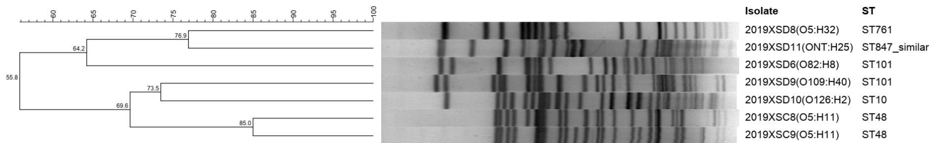
Supplementary Figure S1. PFGE pattern for seven tet(X4) positive tigecycline-resistant isolates.
