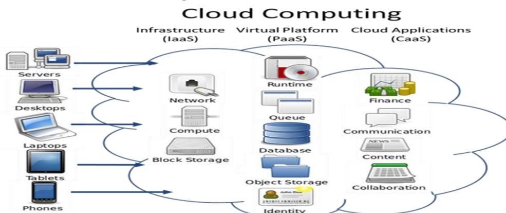
Fig 1. Cloud Computing.
