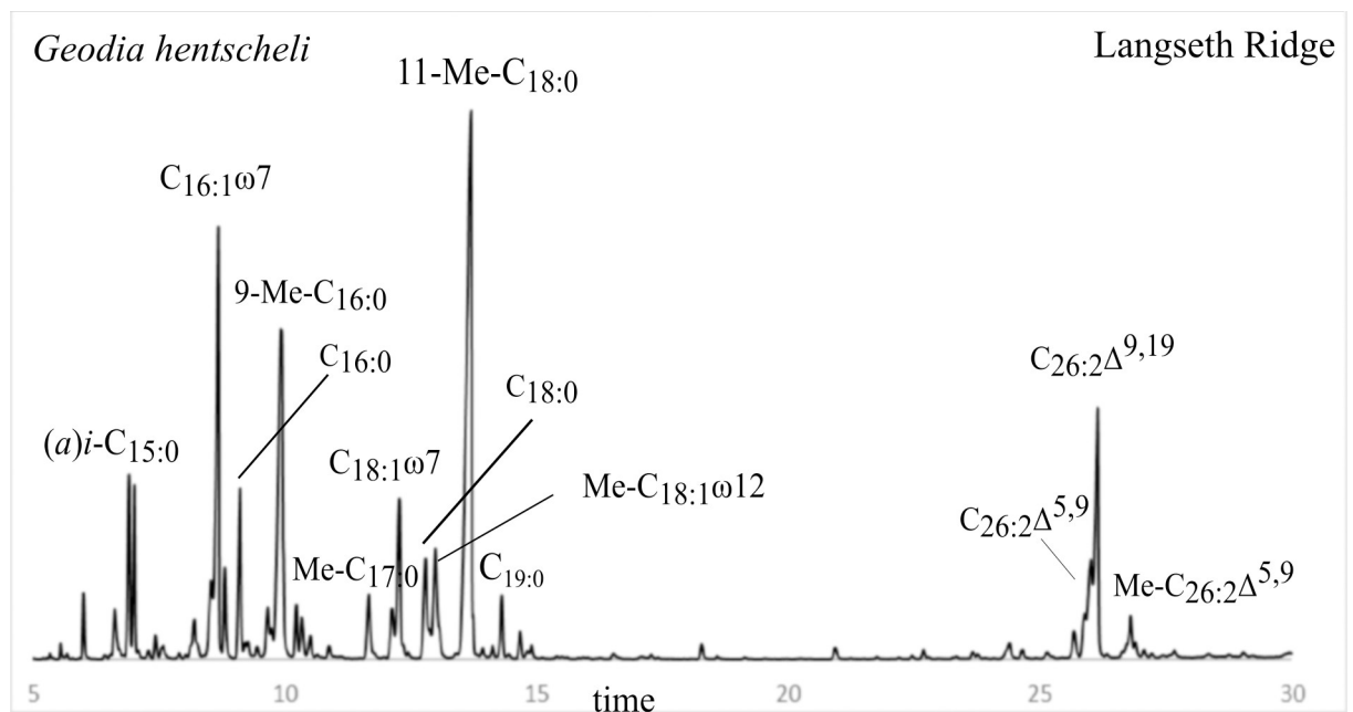
Fig 2. GC trace of the FAME fraction extracted from dem sponge G. hentscheli from Langseth Ridge (Central Arctic). LCFA isomers often co-eluted or were at least not well separated as shown in this PLFA profile for \text{C}_{26:2}\Delta^{5,9} and \text{C}_{26:2}\Delta^{9,19} .
