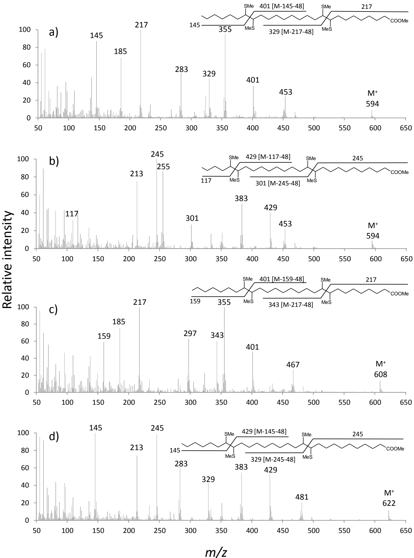
Fig. S1: Mass spectra of DMDS conducts of C 26 (a,b) and C 28 (c,d) LCFA with \Delta^{9,19} (a,c) and \Delta^{11,21} (b,d) unsaturation
