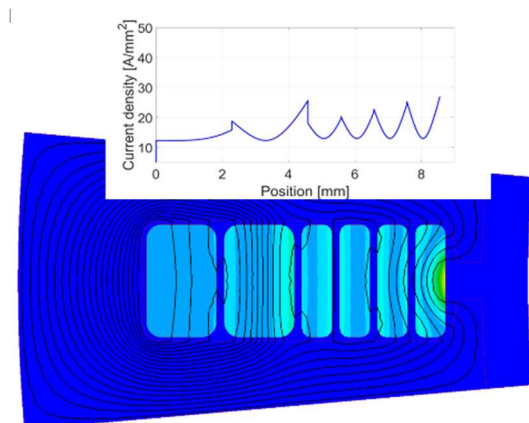
Fig. 8 Parallel conductors
